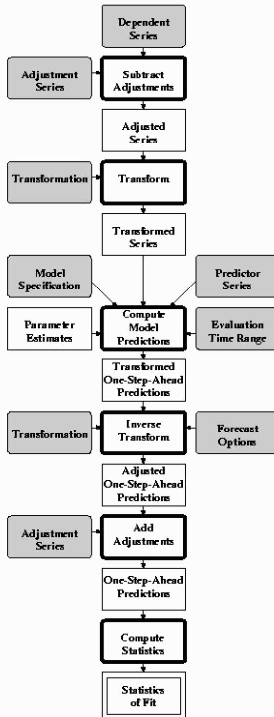
Figure 63.2 Model Evaluation Flow Diagram
