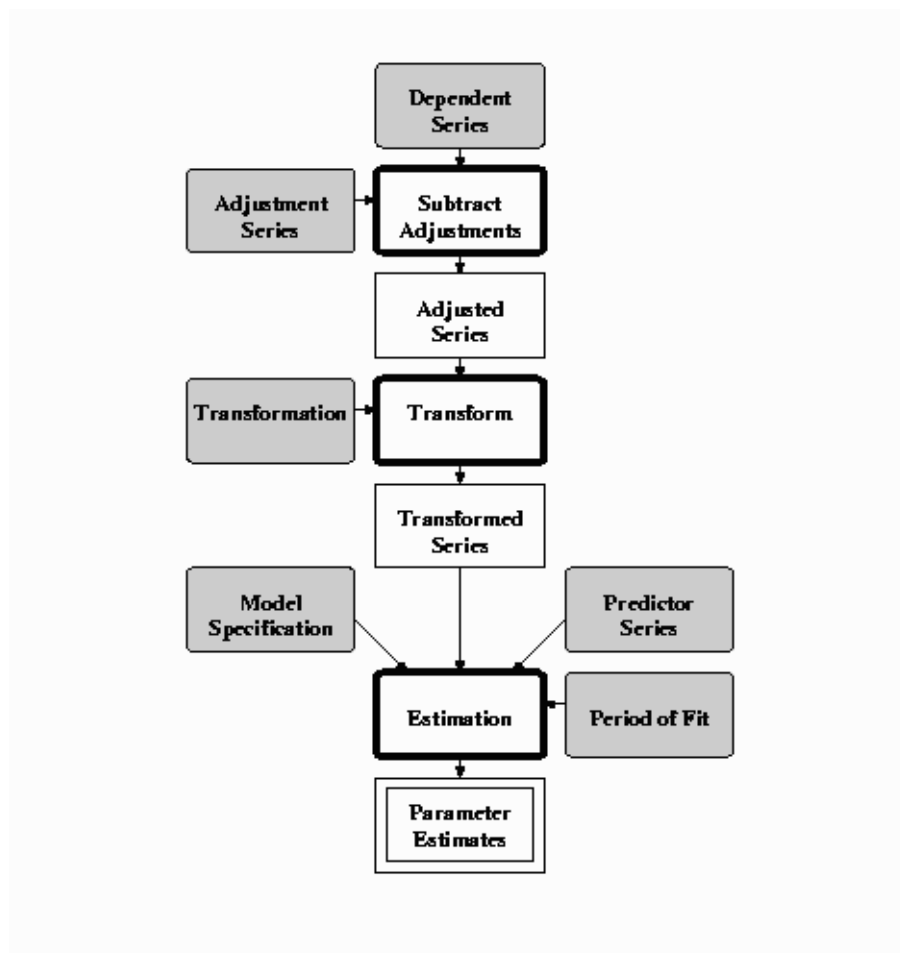
Figure 63.1 Model Fitting Flow Diagram
