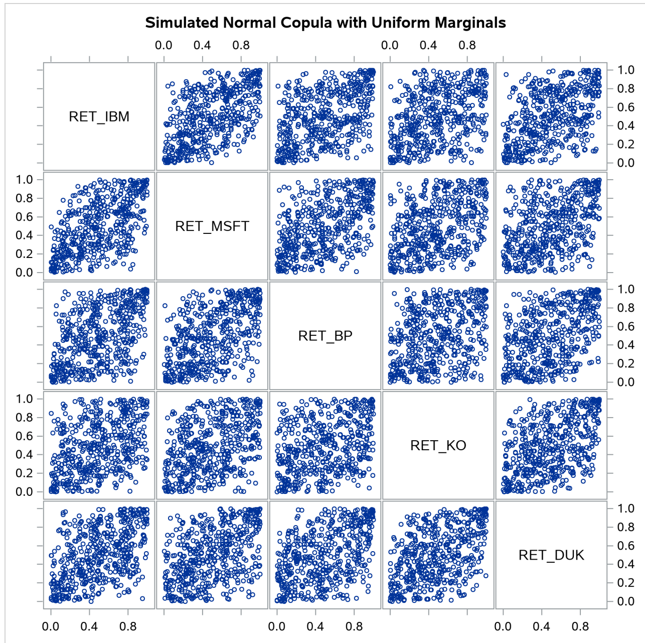
Figure 11.3 Simulated Data, Uniform Marginals
