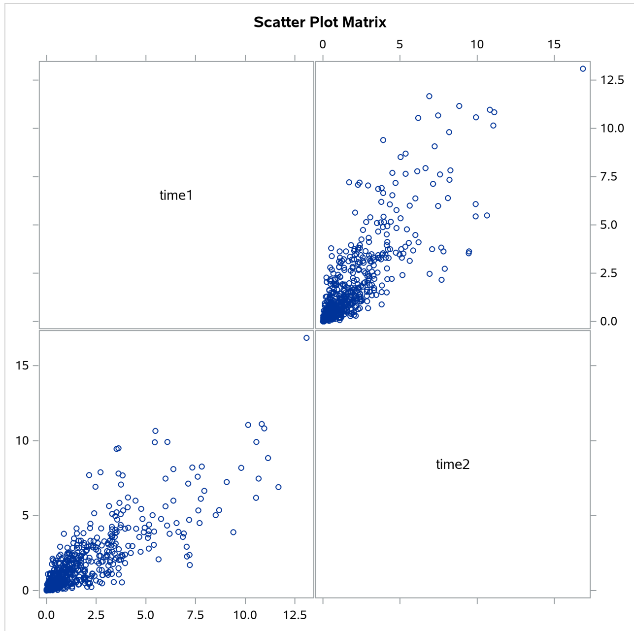
Output 11.2.5 Default Times
