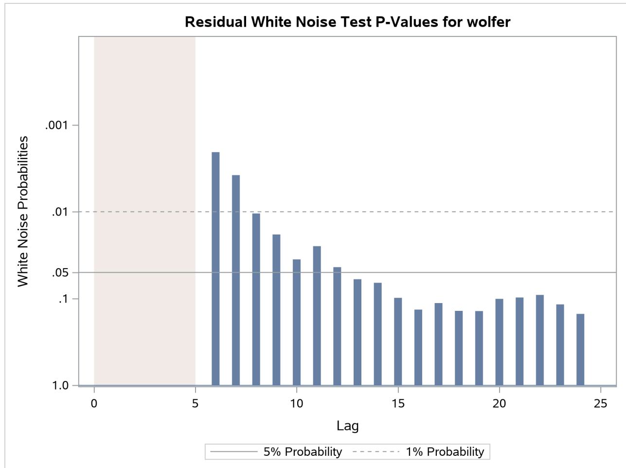
Figure 41.11 Sunspots Series: Ljung-Box Portmanteau Test
