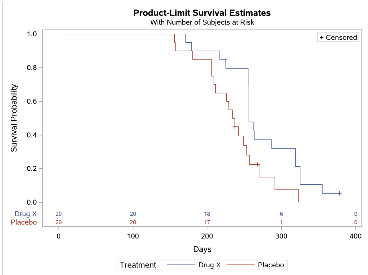
Figure 77.6 Plot of Estimated Survivor Functions
