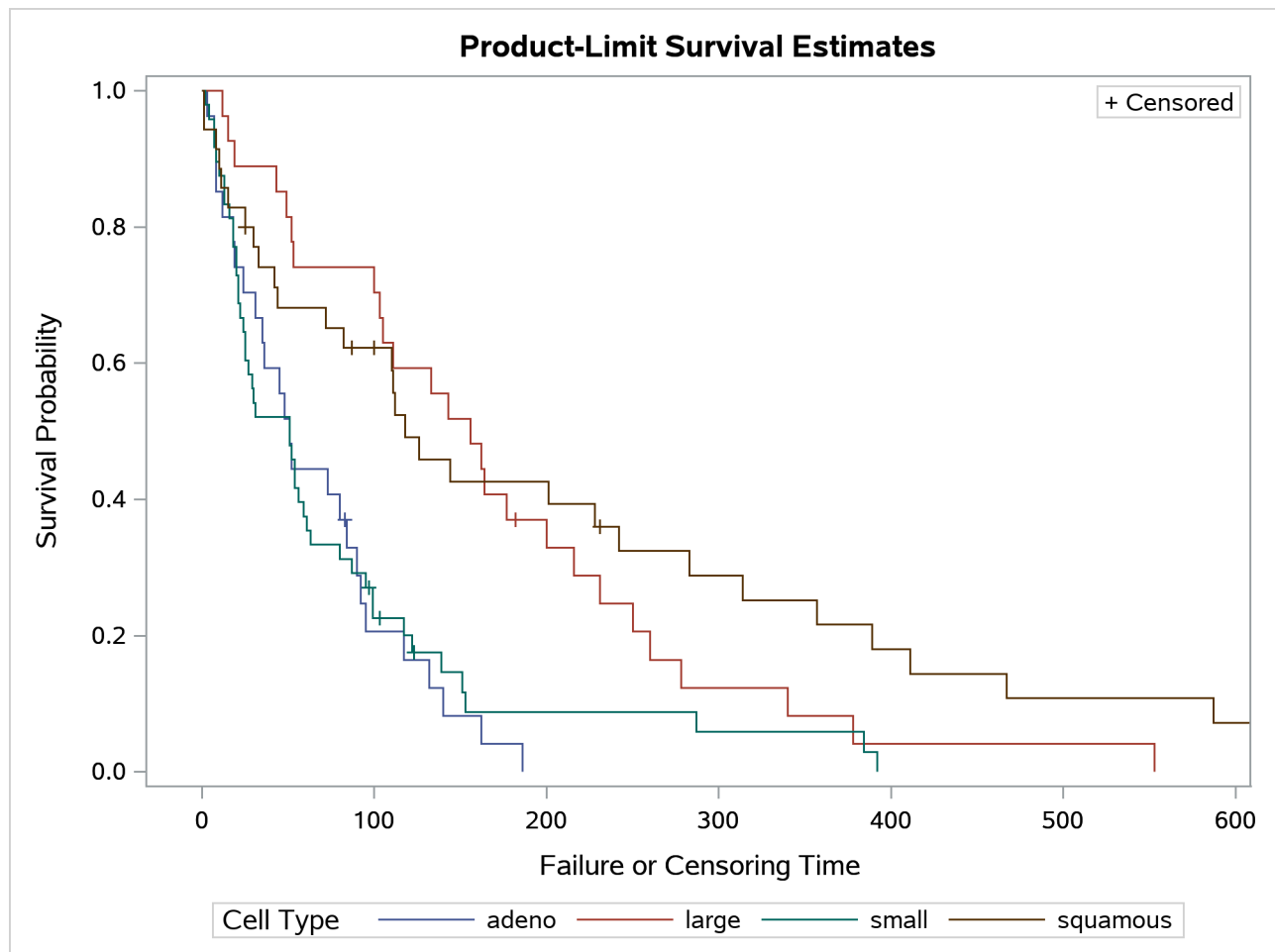
Output 77.1.6 Graph of the Estimated Survivor Functions
