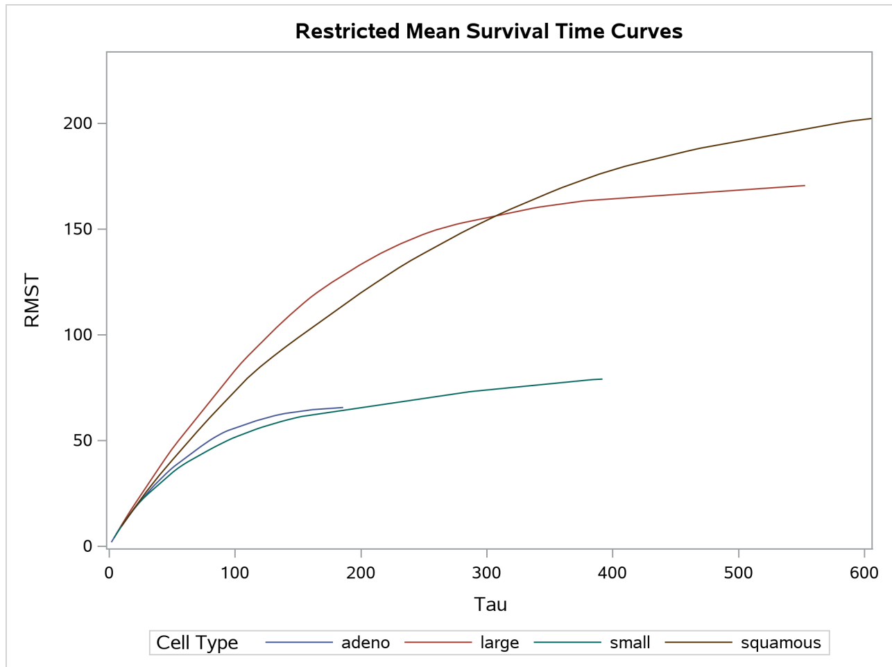
Output 77.5.5 RMST Curves
