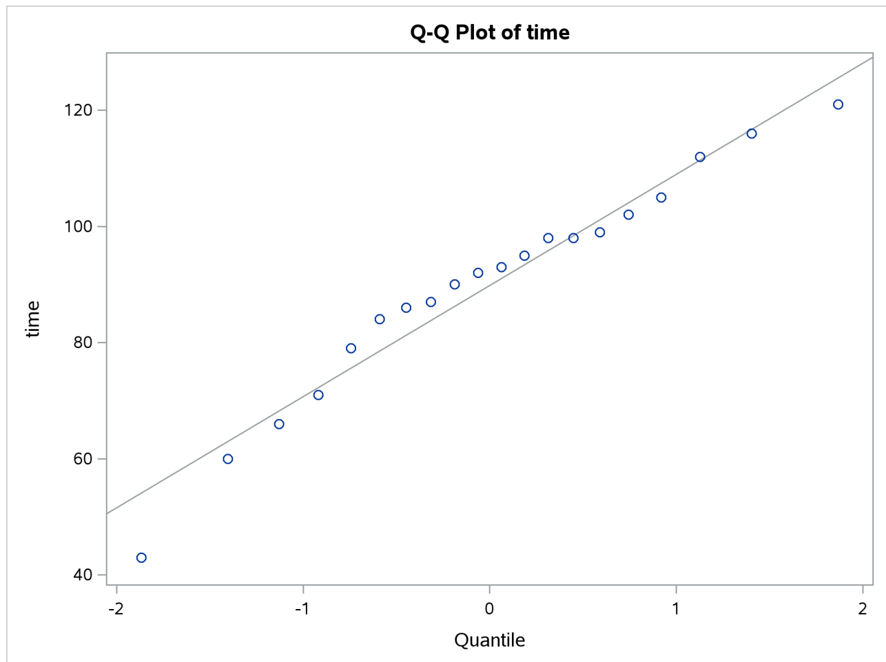
Figure 128.3 Q-Q Plot
