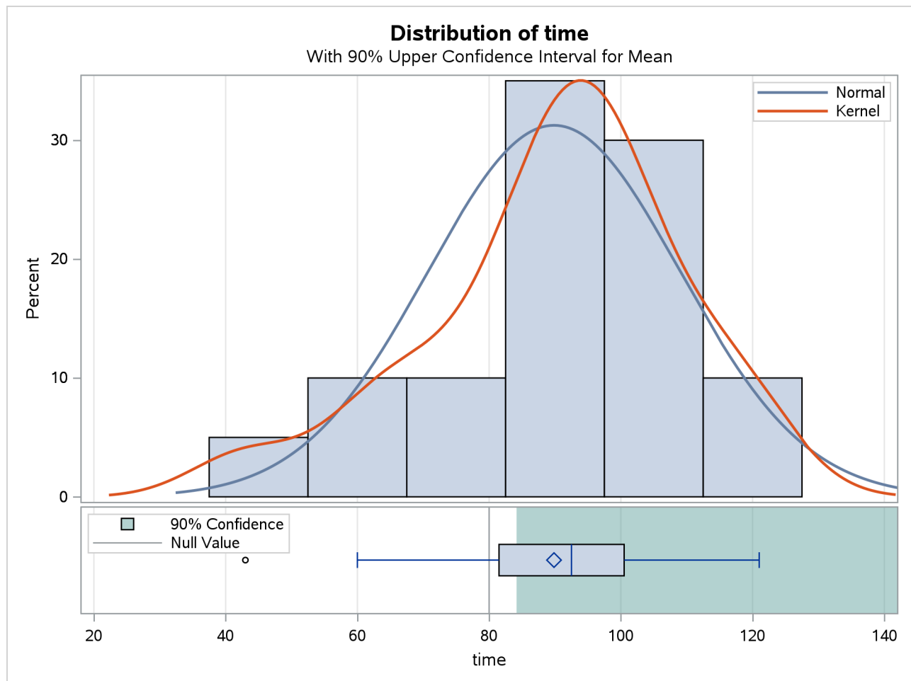
Figure 128.2 Summary Panel
