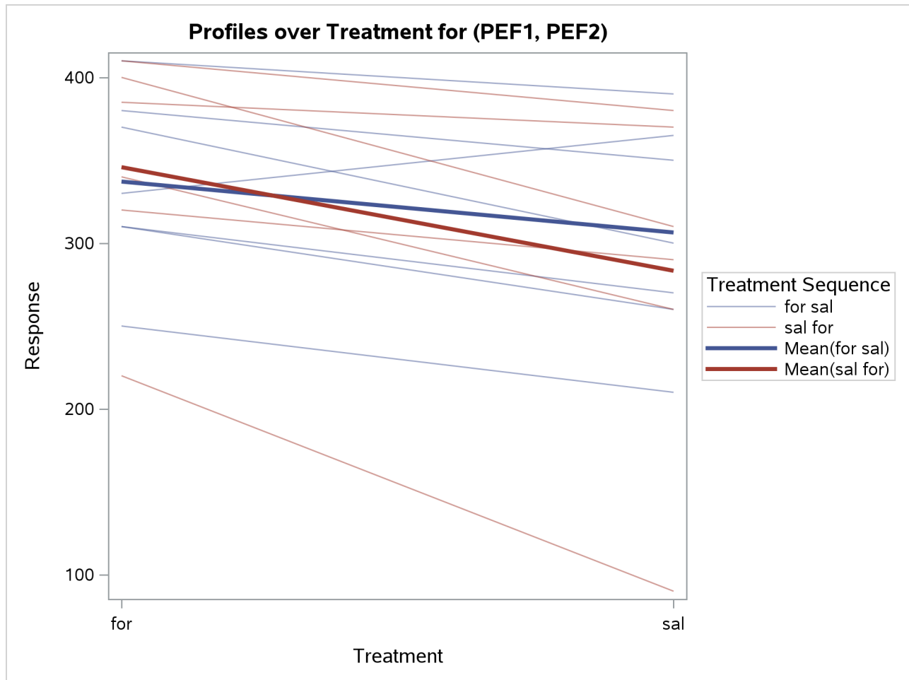
Output 128.4.10 Profiles over Treatment
