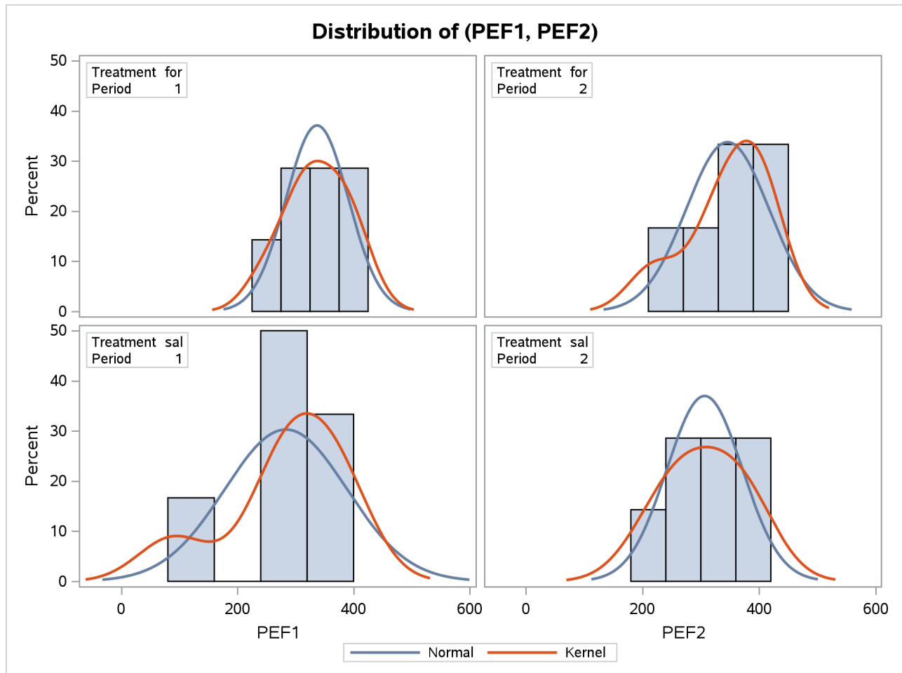
Output 128.4.7 Comparative Histograms
