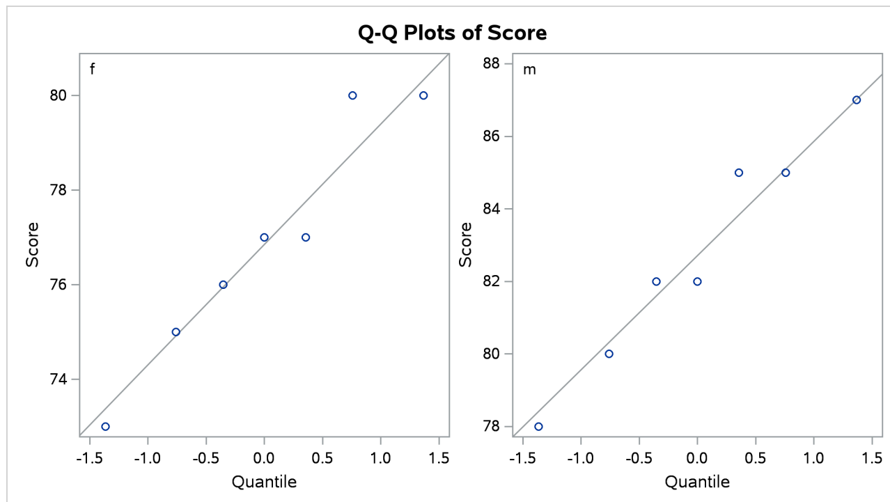
Figure 128.9 Q-Q Plot
