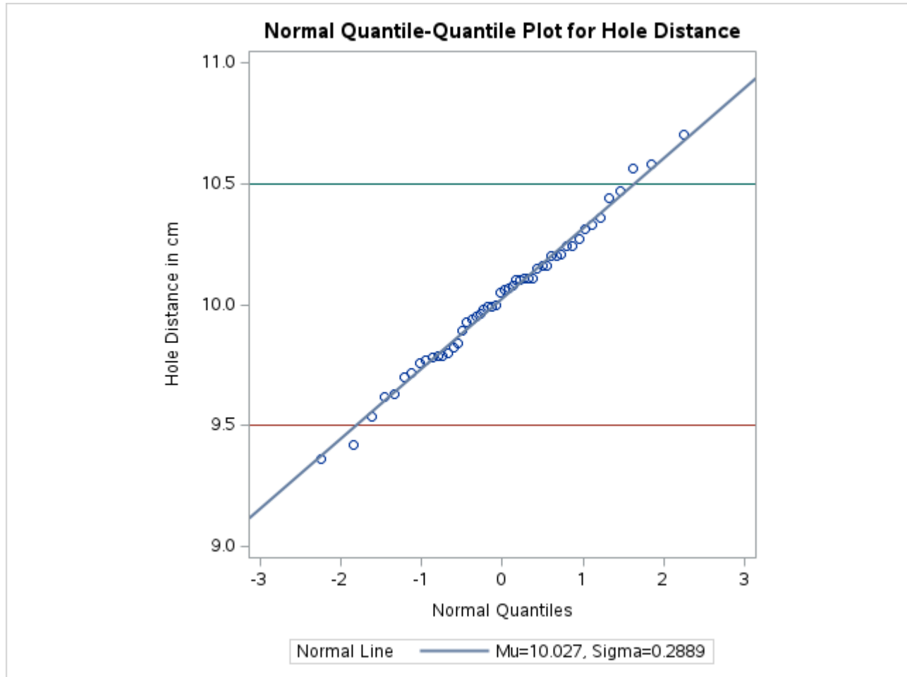
Figure 5.39 Adding a Distribution Reference Line to a Q-Q Plot
