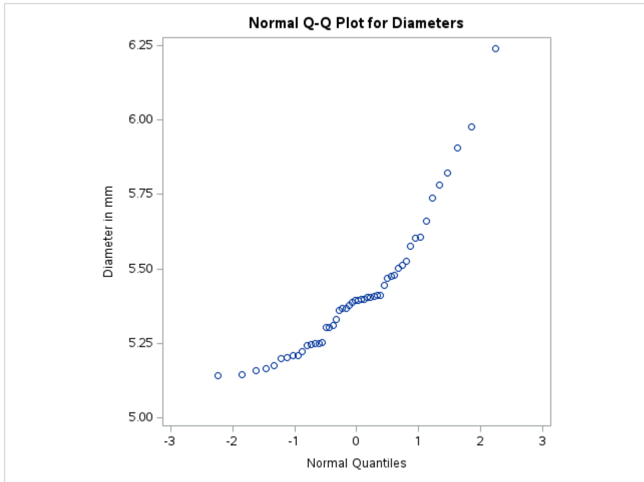
Output 5.23.1 Normal Quantile-Quantile Plot of Nonnormal Data
