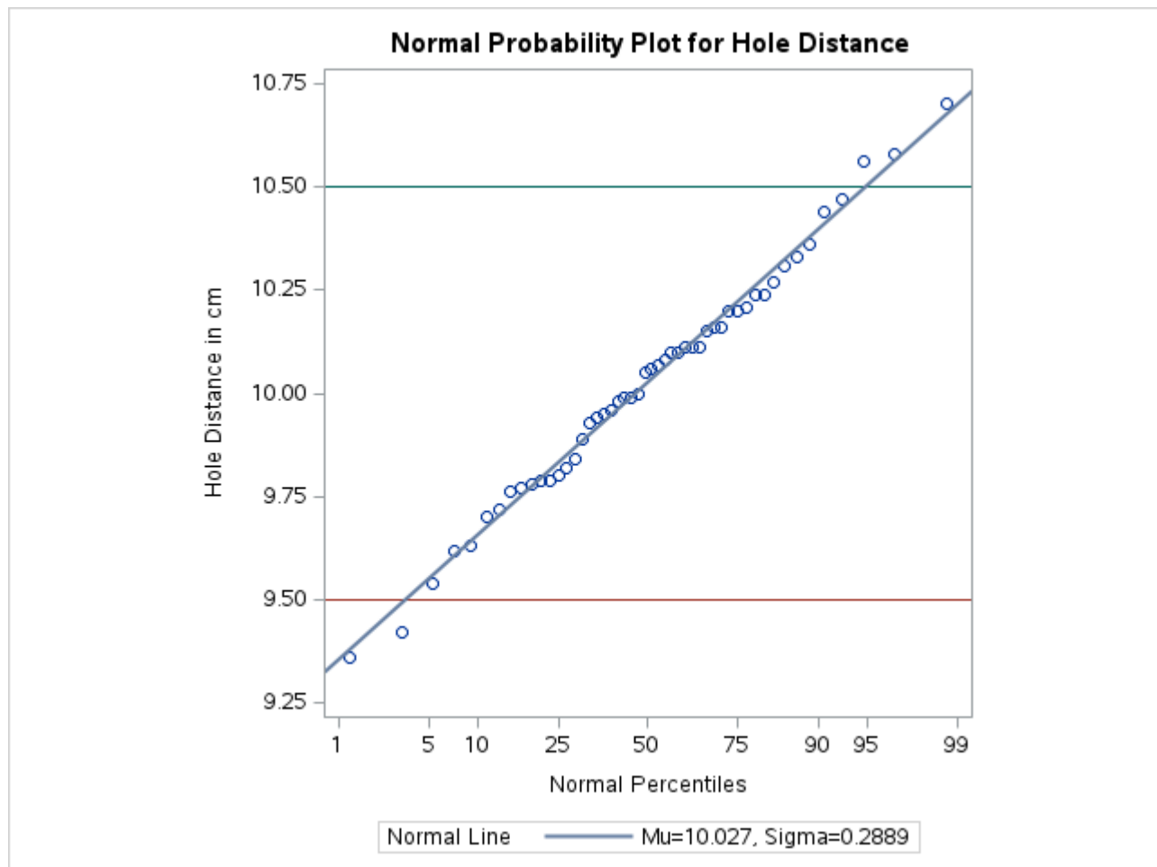
Output 5.21.1 Normal Reference Line
