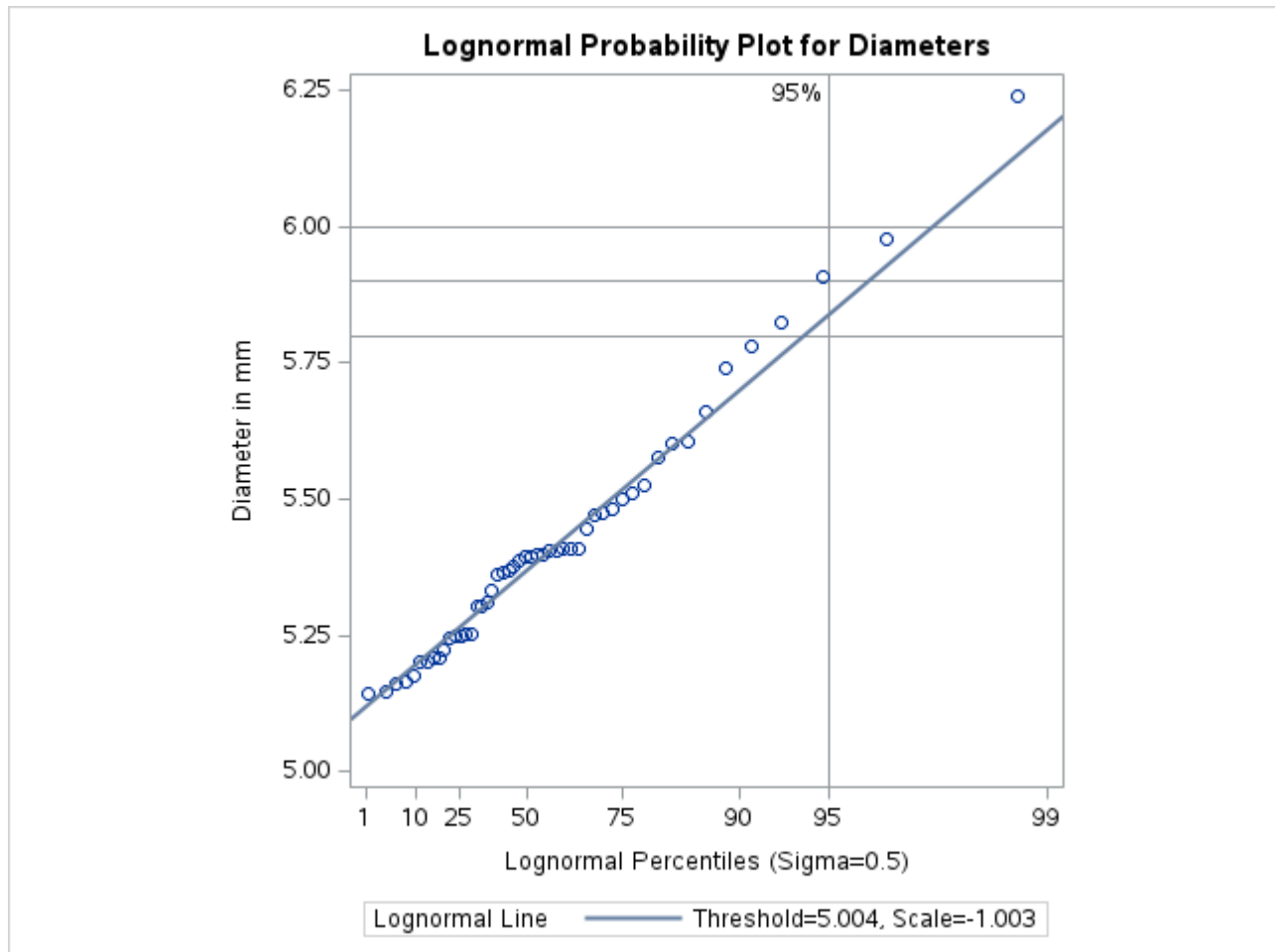
Output 5.22.1 Lognormal Reference Line
