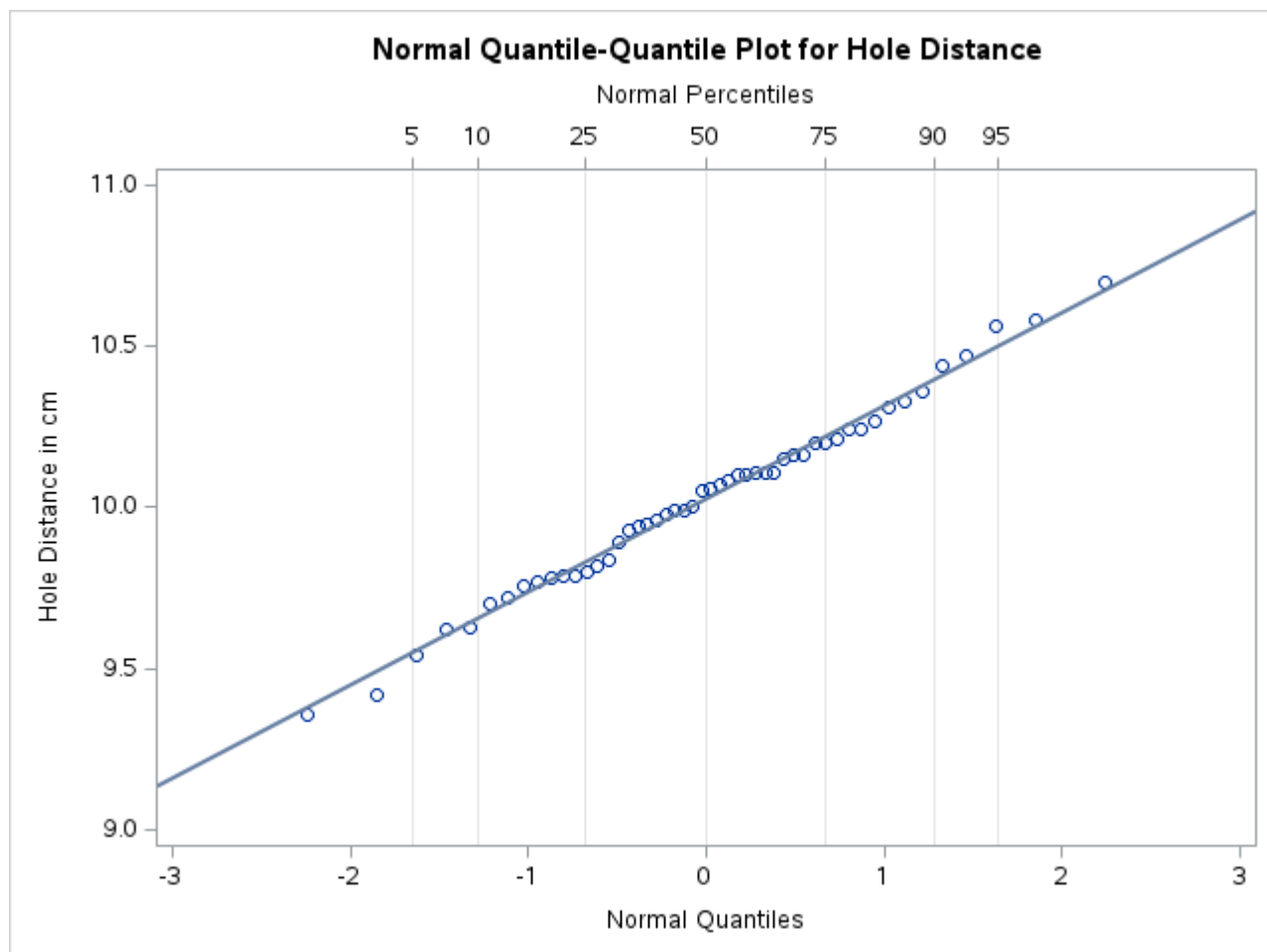
Figure 5.40 Normal Q-Q Plot with Percentile Axis
