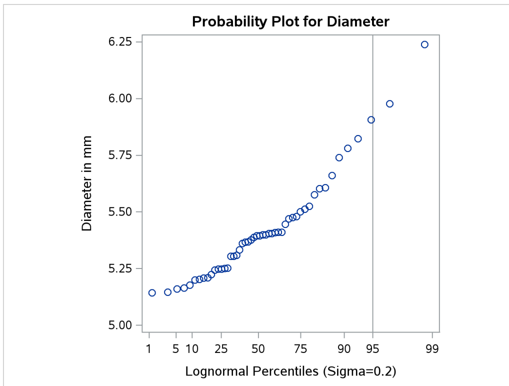
Figure 5.34 Probability Plot Based on Lognormal Distribution with \sigma = 0.2
