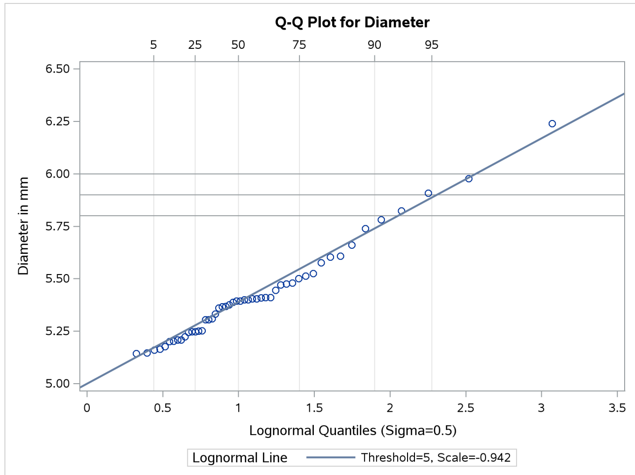
Output 5.24.4 Lognormal Q-Q Plot Identifying Percentiles
