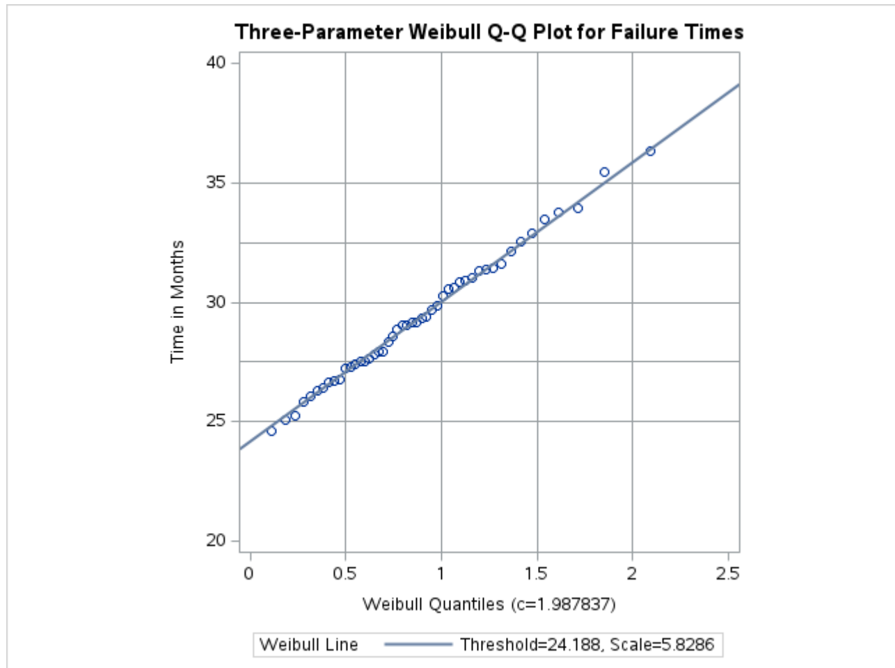
Output 5.25.1 Three-Parameter Weibull Q-Q Plot for c = 2
