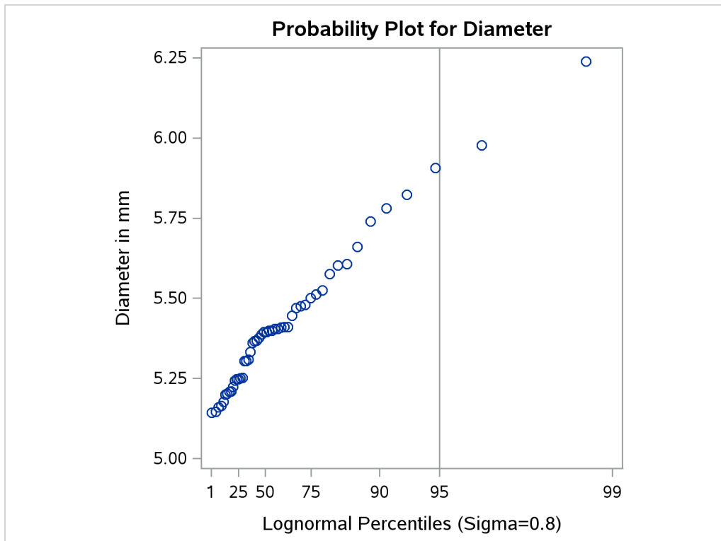
Figure 5.36 Probability Plot Based on Lognormal Distribution with \sigma = 0.8
