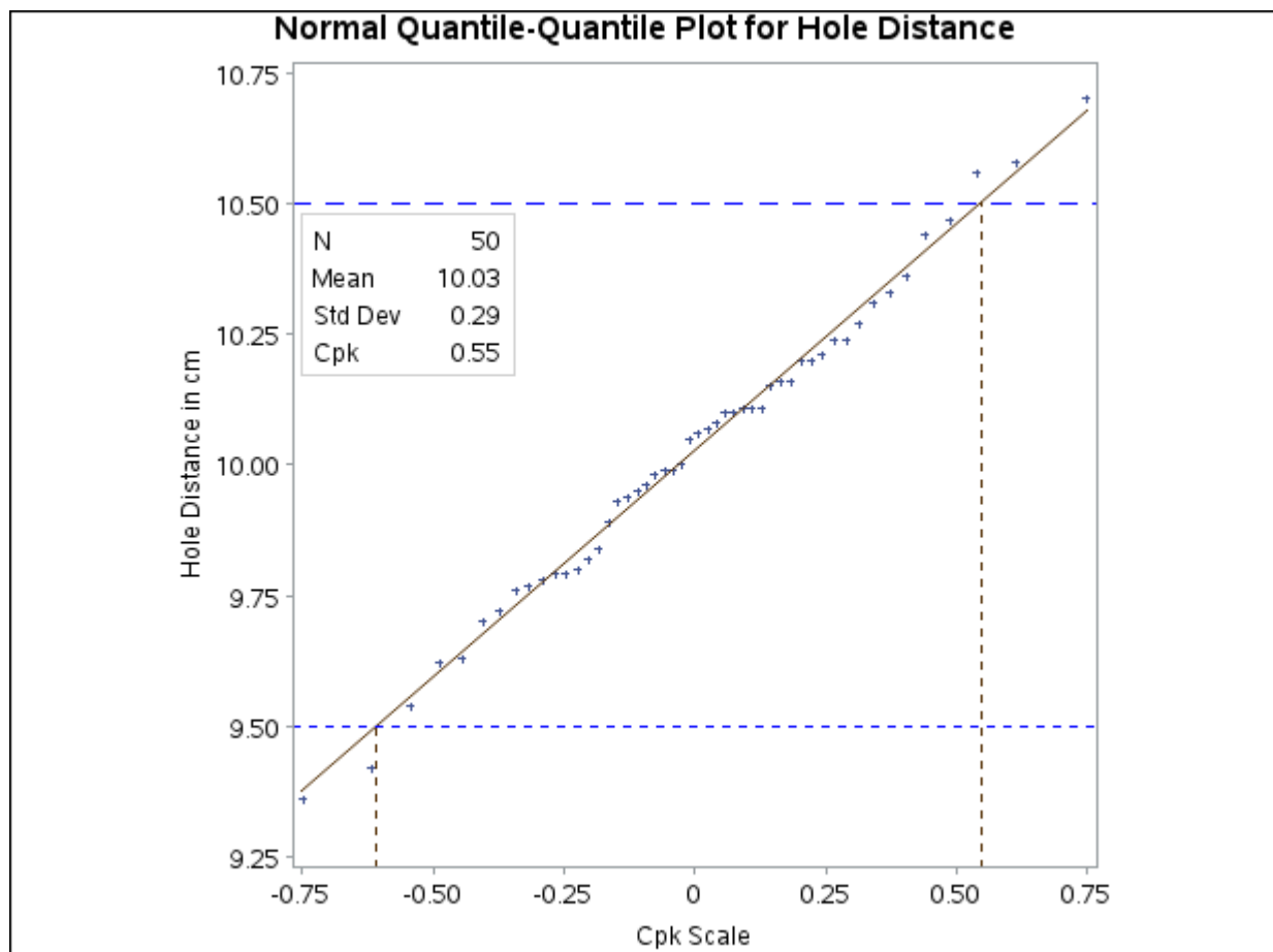
Output 5.26.1 Normal Q-Q Plot With C_{pk} Scaling
