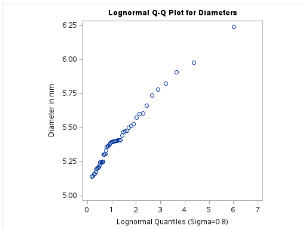
Output 5.24.3 Lognormal Quantile-Quantile Plot ( \sigma = 0.8 )
