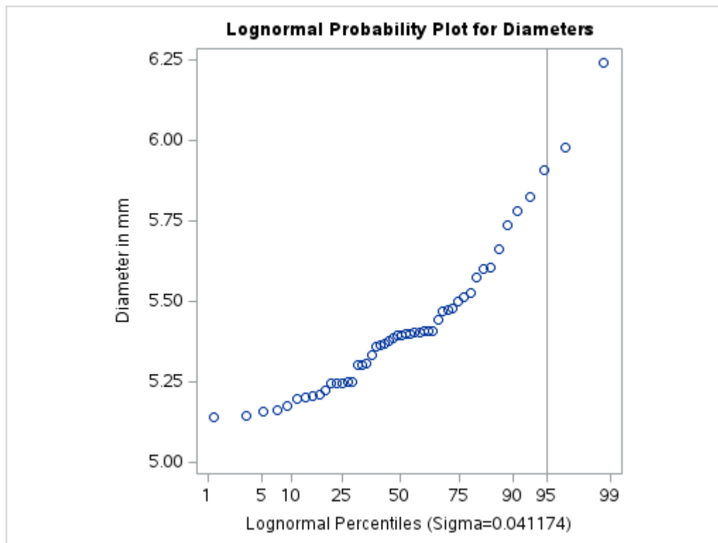
Figure 5.37 Probability Plot Based on Lognormal Distribution with Estimated \sigma
