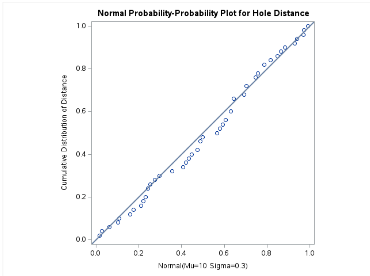
Figure 5.30 Normal P-P Plot with Diagonal Reference Line
