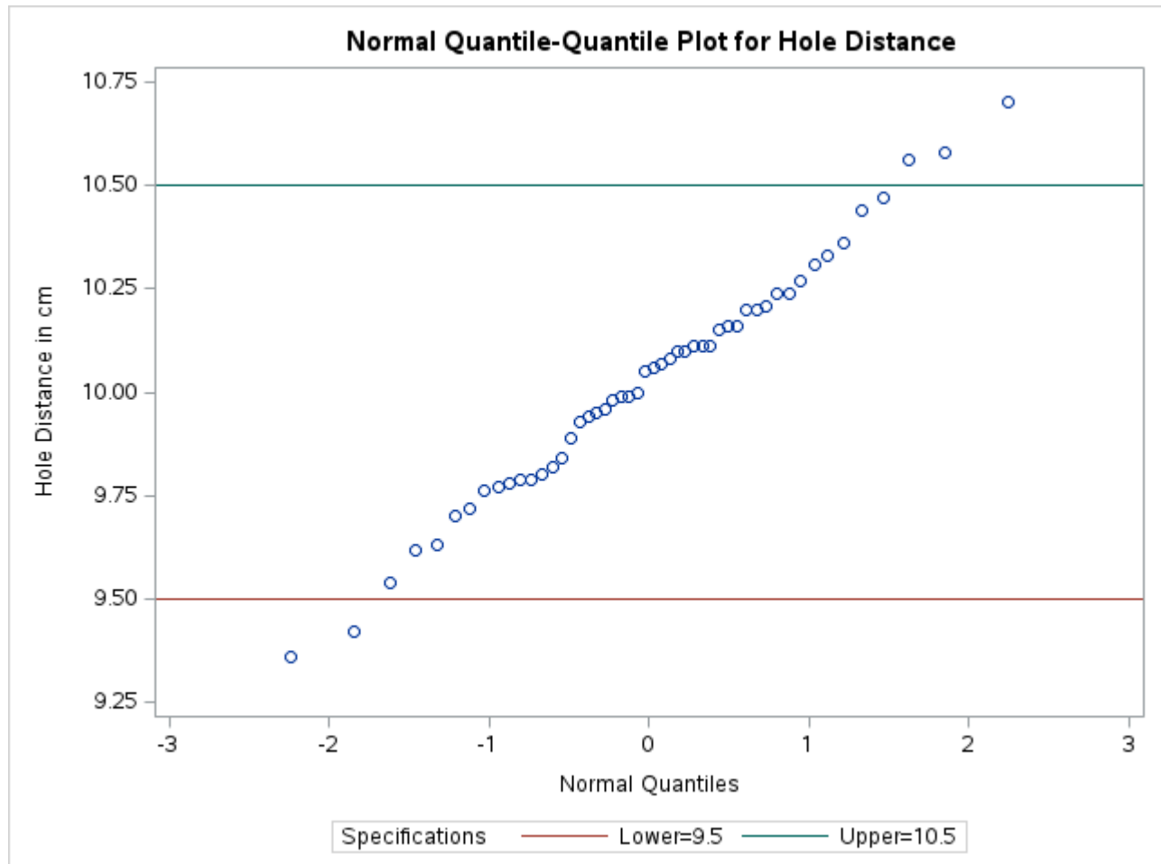
Figure 5.38 Normal Quantile-Quantile Plot Created with Traditional Graphics
