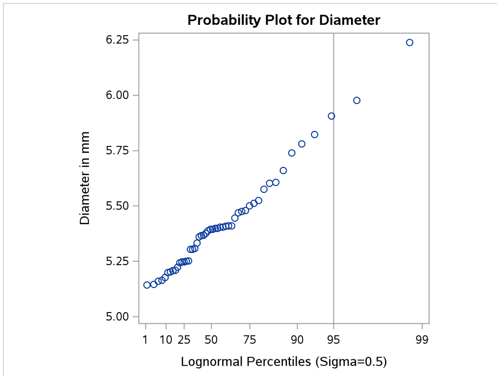
Figure 5.35 Probability Plot Based on Lognormal Distribution with \sigma = 0.5
