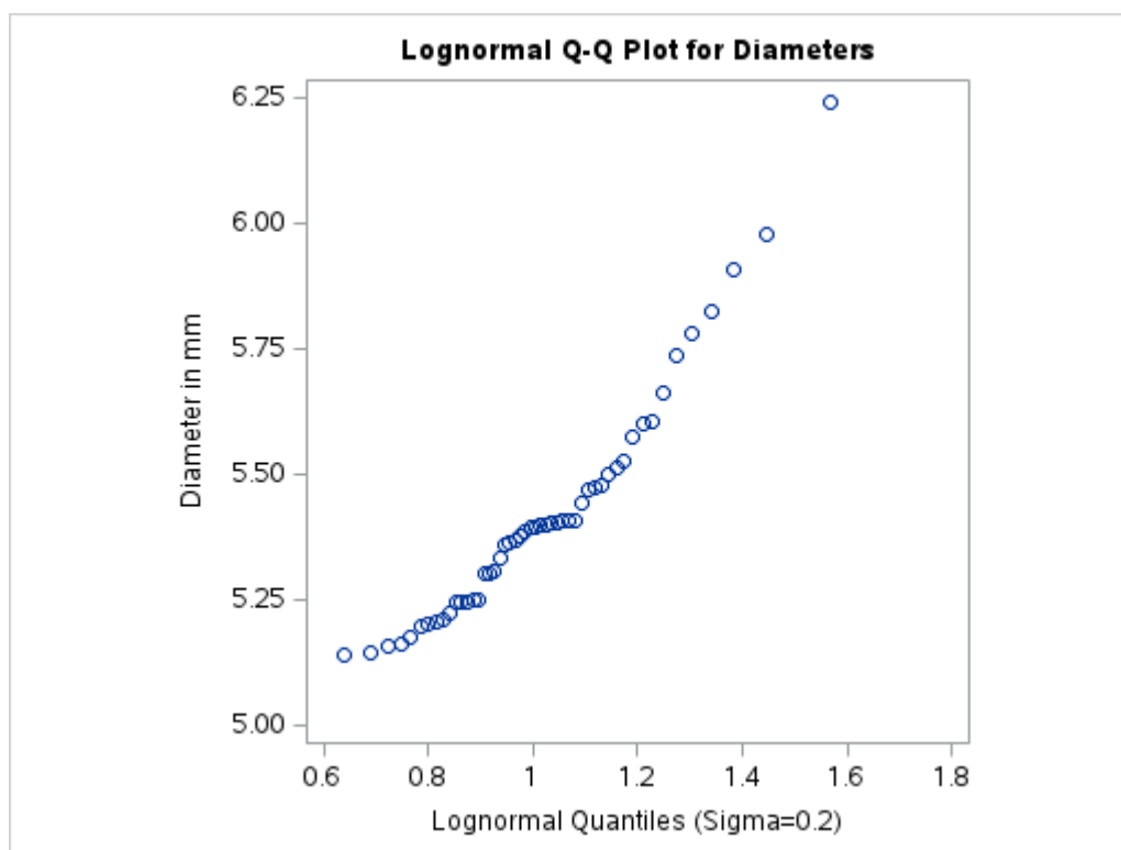
Output 5.24.1 Lognormal Quantile-Quantile Plot ( \sigma=0.2 )
