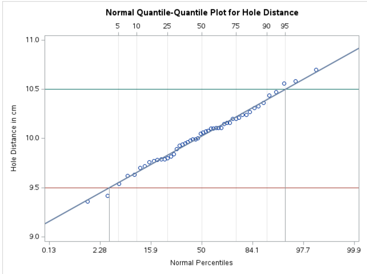
Figure 5.41 Normal Q-Q Plot for Reading Percentiles of Specification Limits
