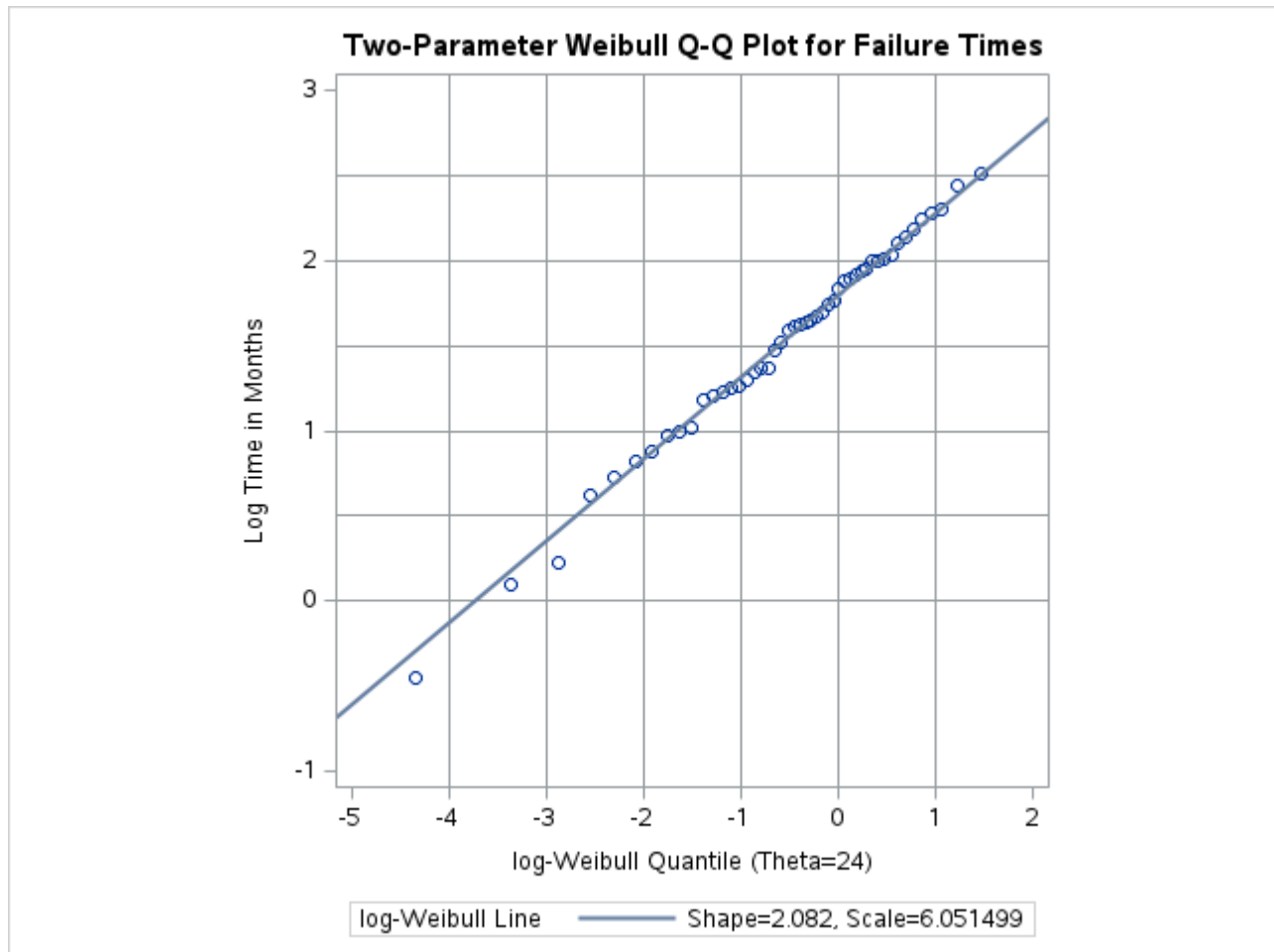
Output 5.25.2 Two-Parameter Weibull Q-Q Plot for \theta_0 = 24
