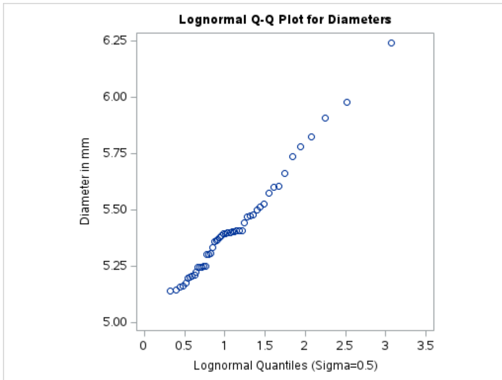
Output 5.24.2 Lognormal Quantile-Quantile Plot ( \sigma = 0.5 )
