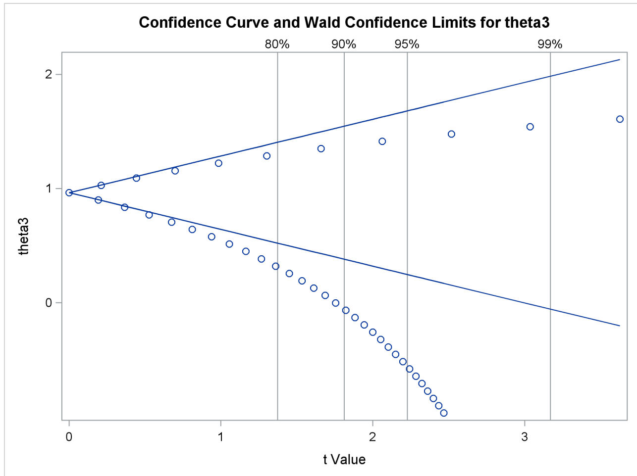
Output 82.7.5 Confidence Curve
