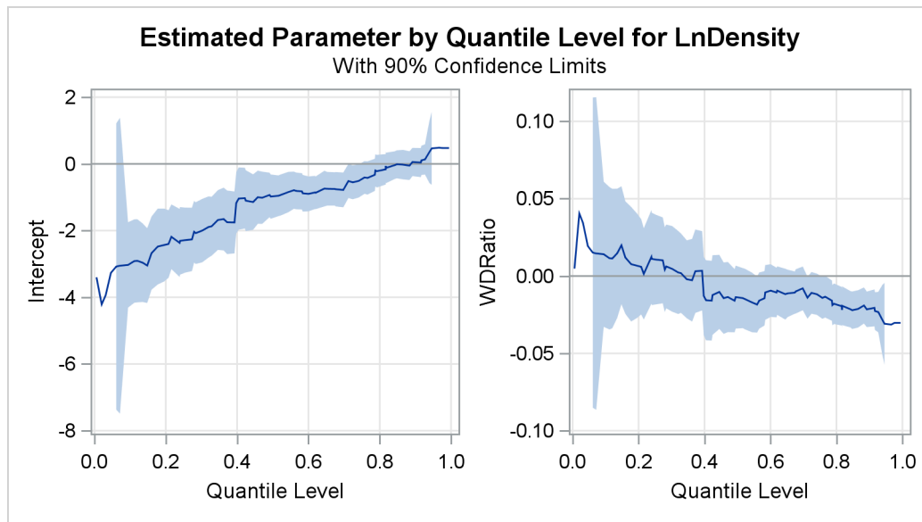
Figure 97.10 Quantile Processes for Intercept and Slope
