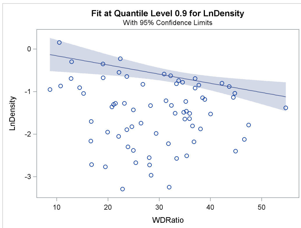
Figure 97.14 Fit Plot with Confidence Limits
