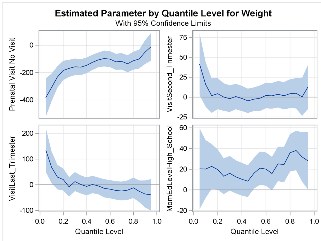
Output 97.3.4 Quantile Processes with 95% Confidence Bands
