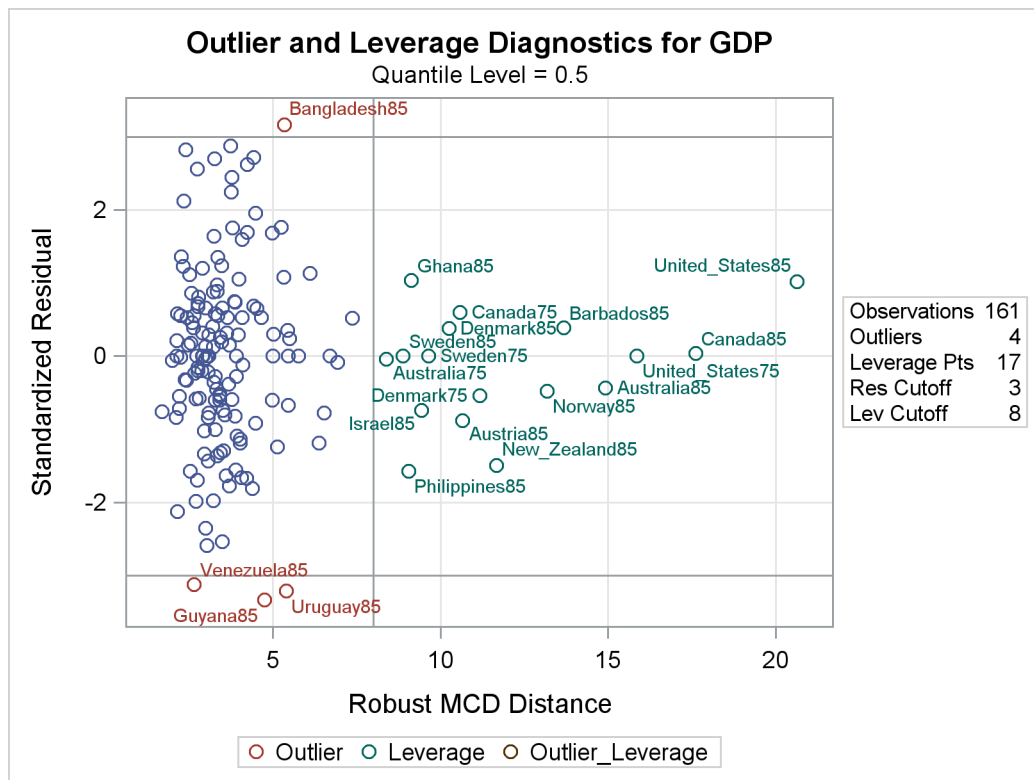
Output 97.2.3 Plot of Residual versus Robust Distance
