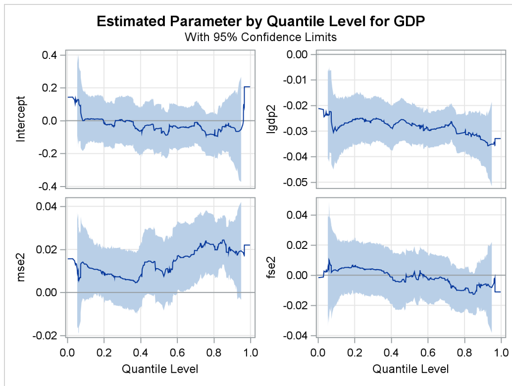
Output 97.2.7 Quantile Processes with 95% Confidence Bands
