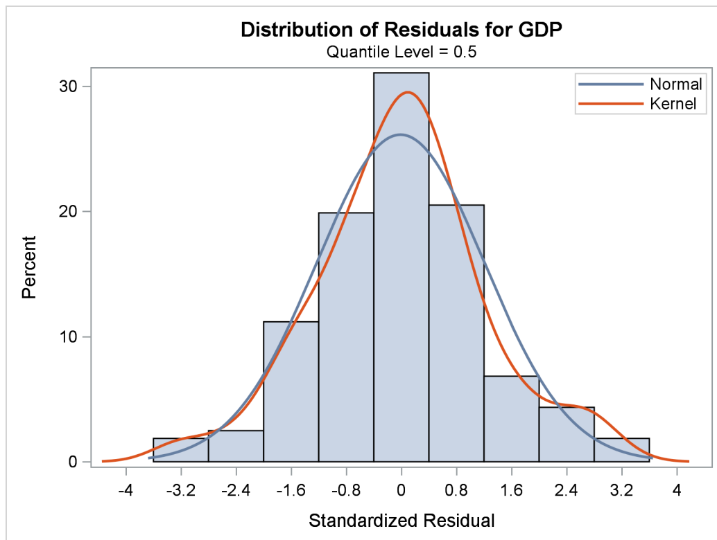
Output 97.2.5 Histogram for Residuals
