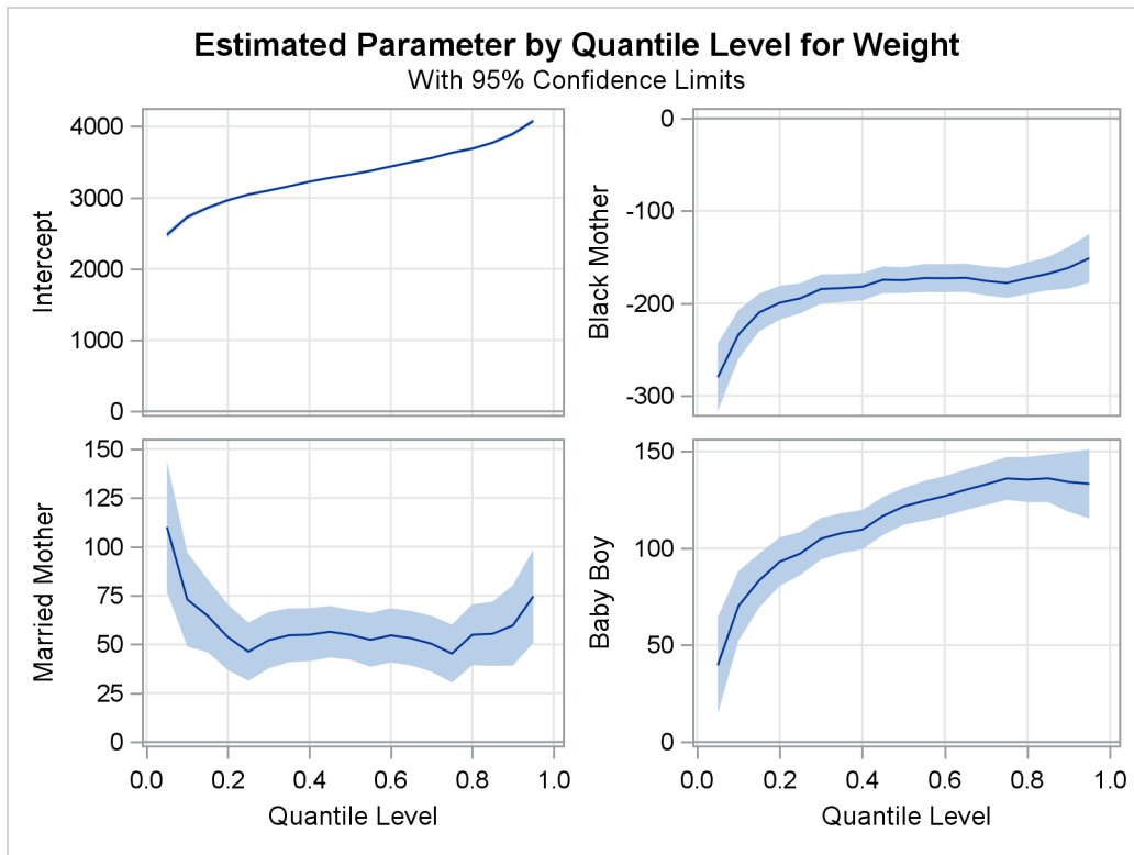
Output 97.3.3 Quantile Processes with 95% Confidence Bands
