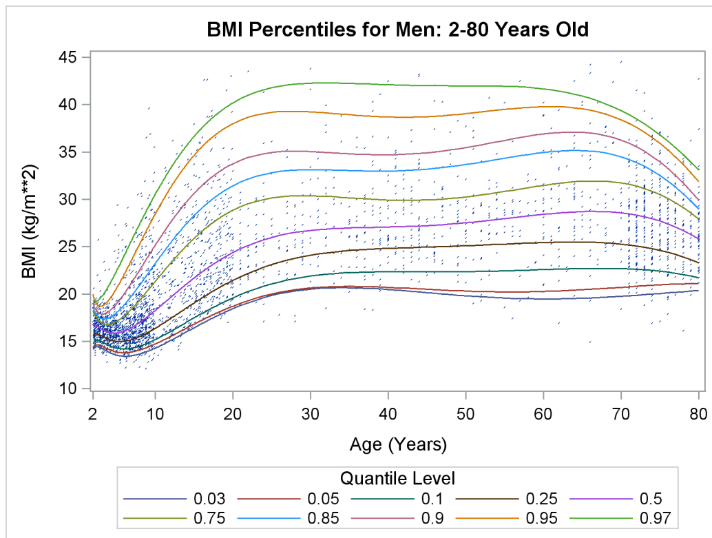
Figure 97.2 Percentiles for Body Mass Index
