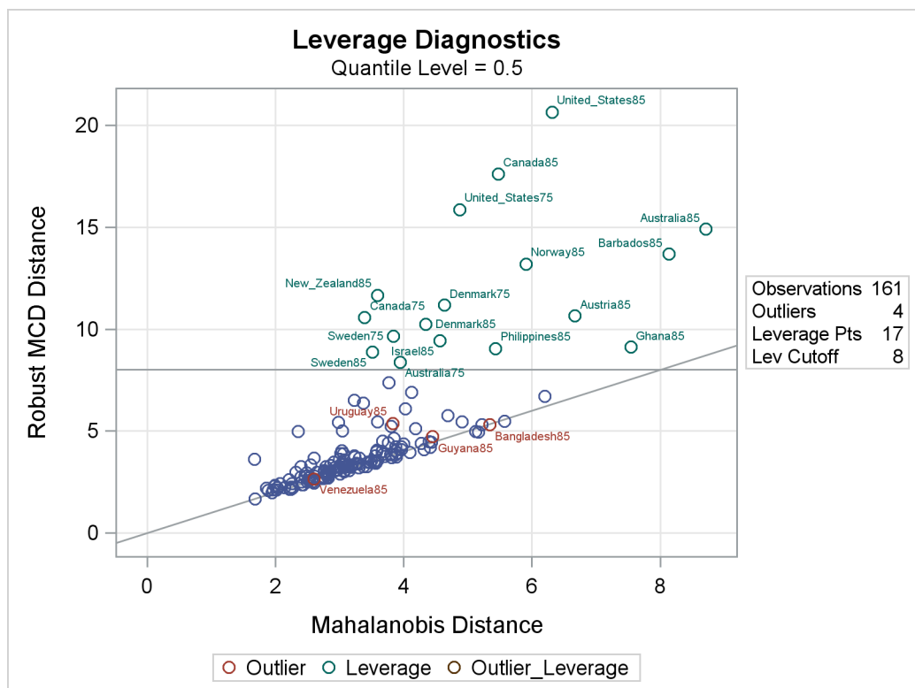
Output 97.2.4 Plot of Robust Distance versus Mahalanobis Distance
