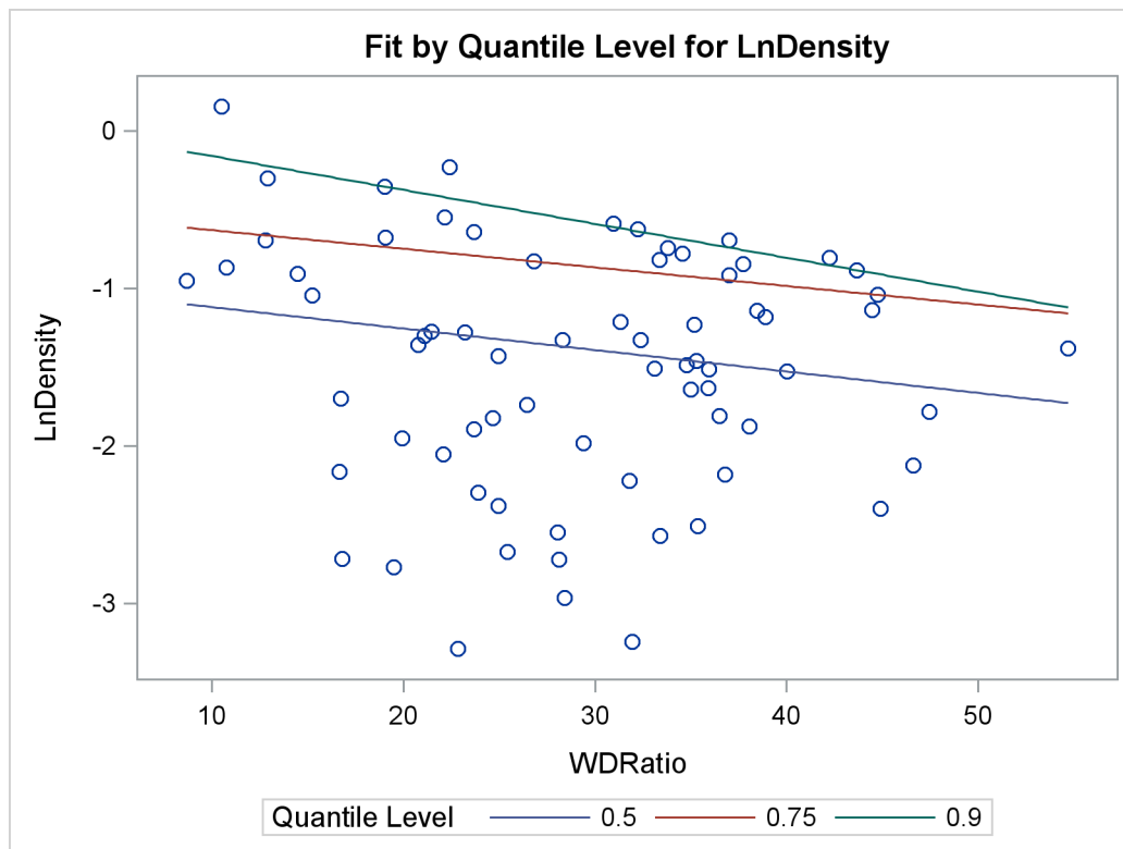
Figure 97.15 Fit Plot for Multiple Quantiles
