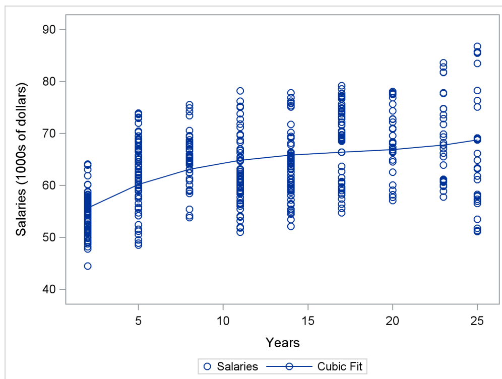
Output 97.5.1 Salary and Years as Professor: Cubic Fit
