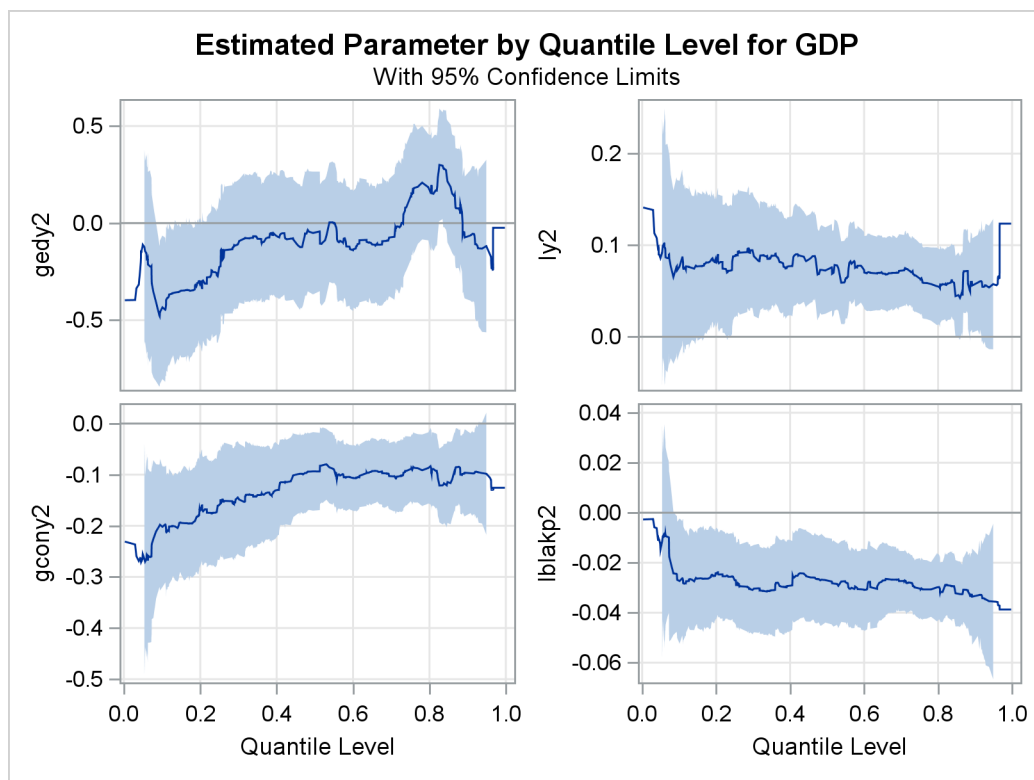
Output 97.2.8 Quantile Processes with 95% Confidence Bands
