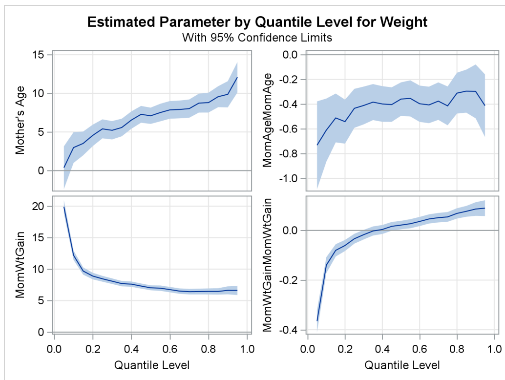
Output 97.3.6 Quantile Processes with 95% Confidence Bands
