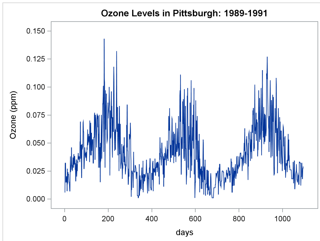
Output 97.4.1 Time Series of Ozone Levels in Pittsburgh, Pennsylvania
