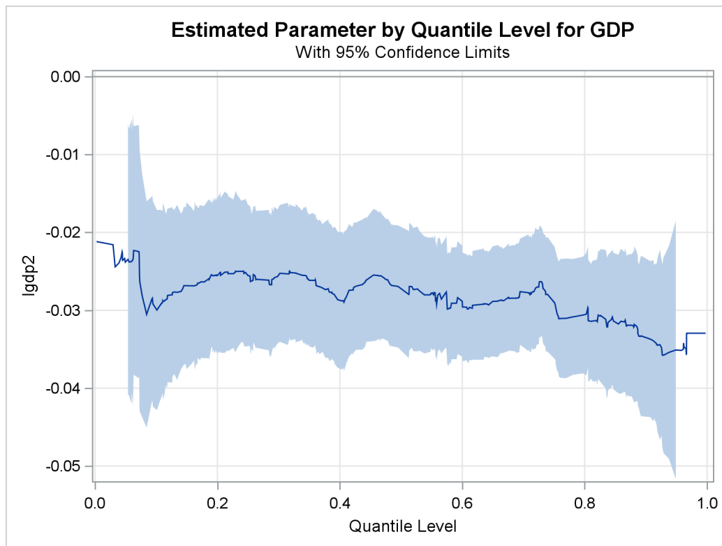
Output 97.2.9 Quantile Process Plot for LGDP2
