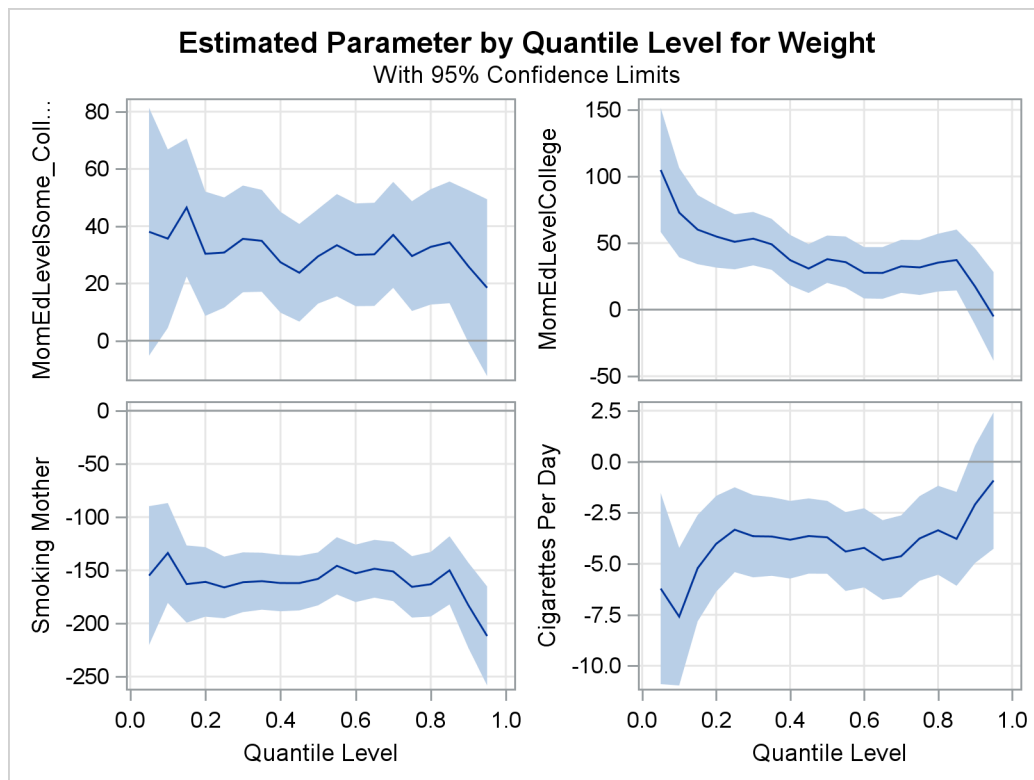
Output 97.3.5 Quantile Processes with 95% Confidence Bands
