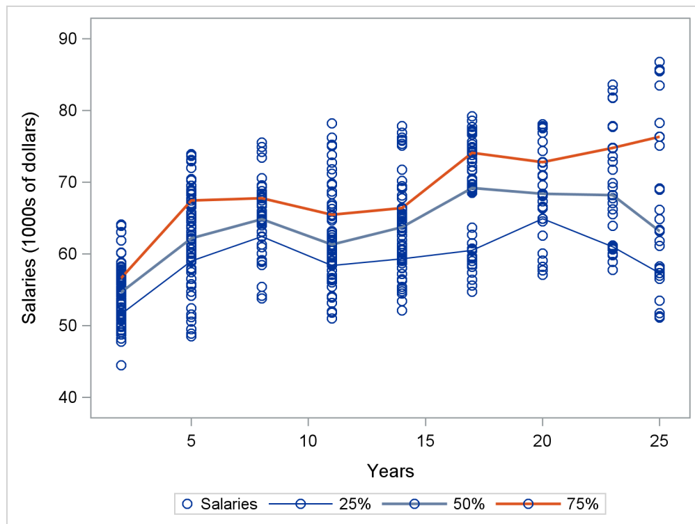
Output 97.5.2 Salary and Years as Professor: Sample Quantiles
