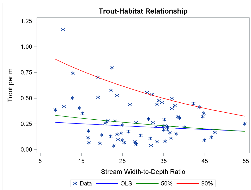
Figure 97.1 Trout Density in Streams
