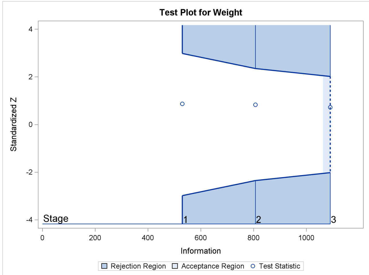
Output 104.2.19 Sequential Test Plot
