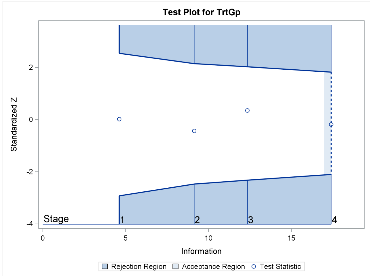
Output 104.7.16 Sequential Test Plot
