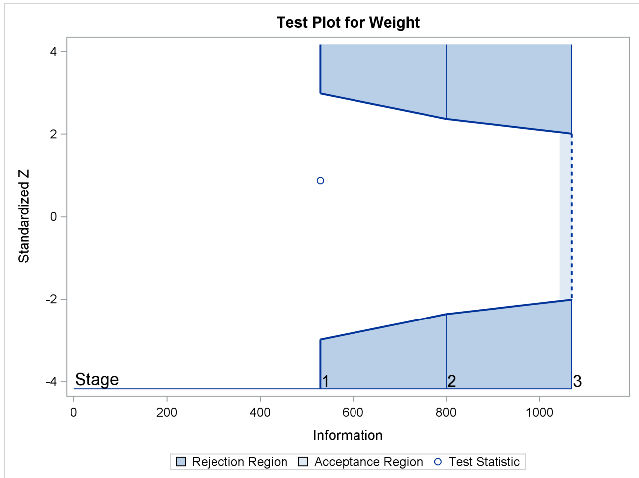
Output 104.2.11 Sequential Test Plot
