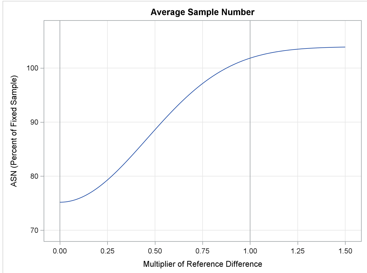
Output 104.3.15 ASN Plot
