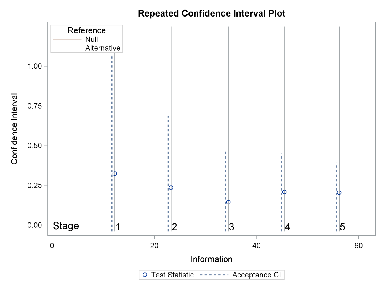
Output 104.5.18 Repeated Confidence Intervals Plot
