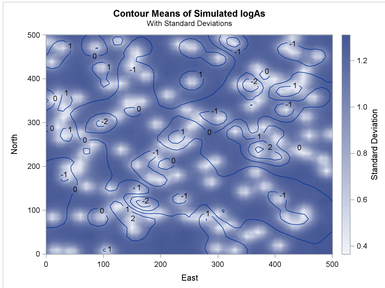
Output 105.3.7 Simulated Arsenic Logarithm Values with Gaussian-Gaussian Covariance
