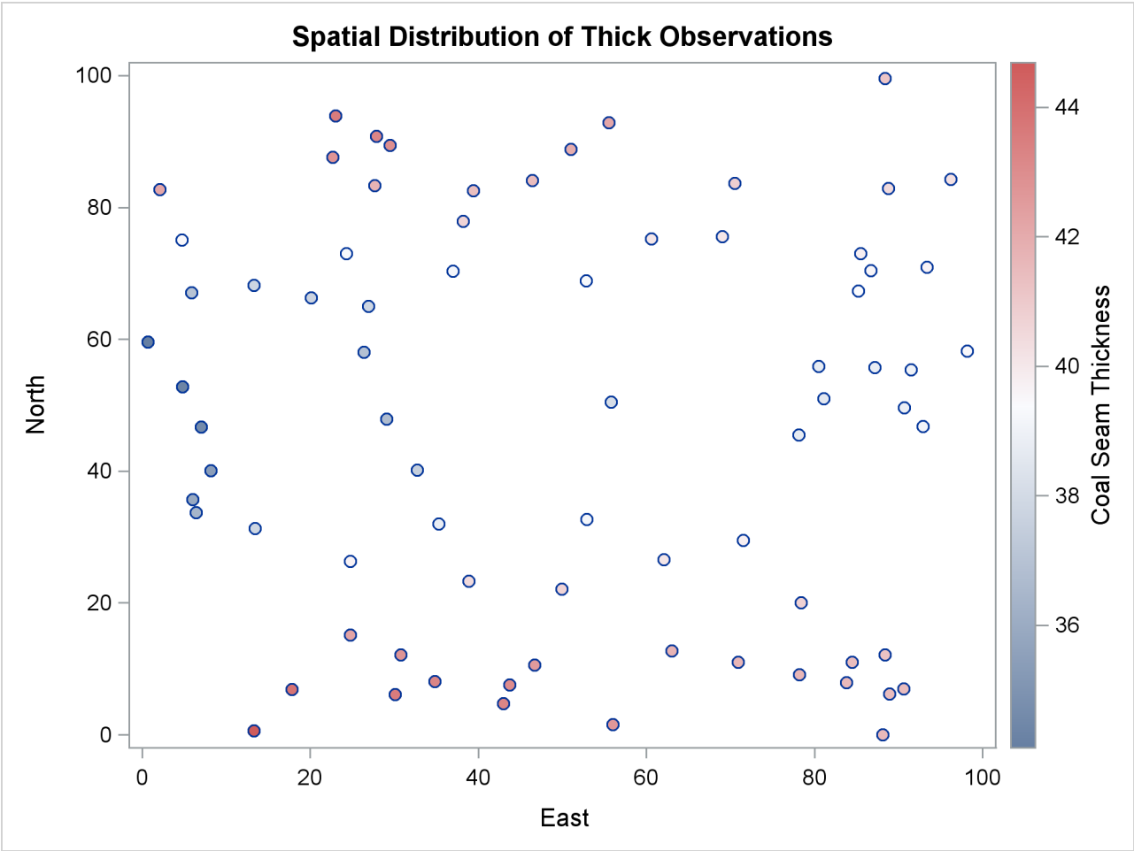
Figure 105.2 Scatter Plot of the Observations Spatial Distribution
