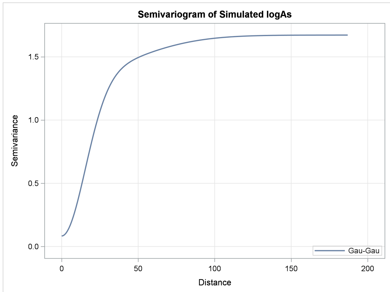
Output 105.3.6 Gaussian-Gaussian Semivariogram Model Used in Simulation
