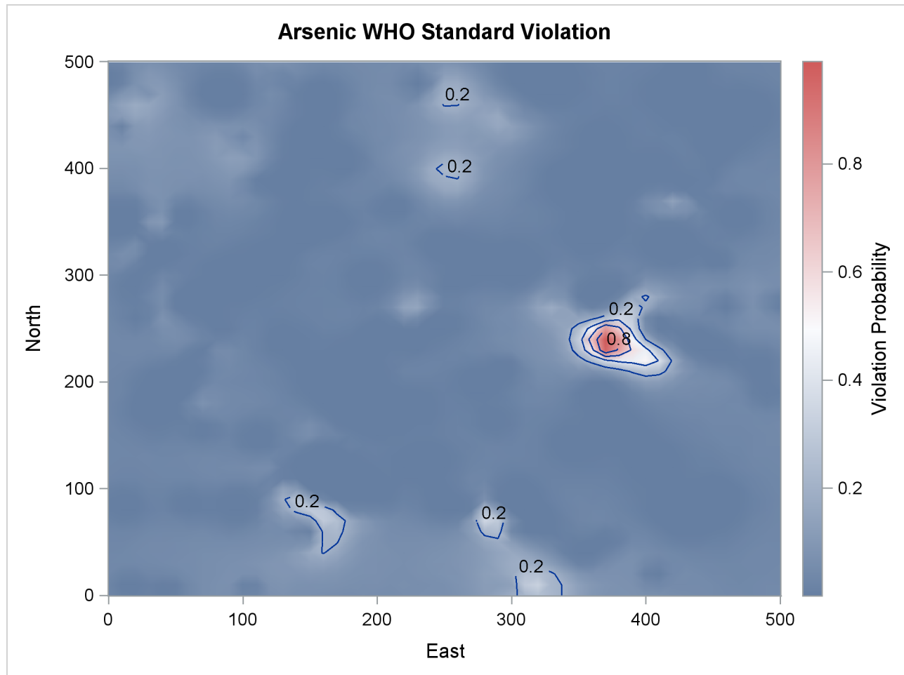
Output 105.3.9 Map of Violation of the Arsenic WHO Standard Probability
