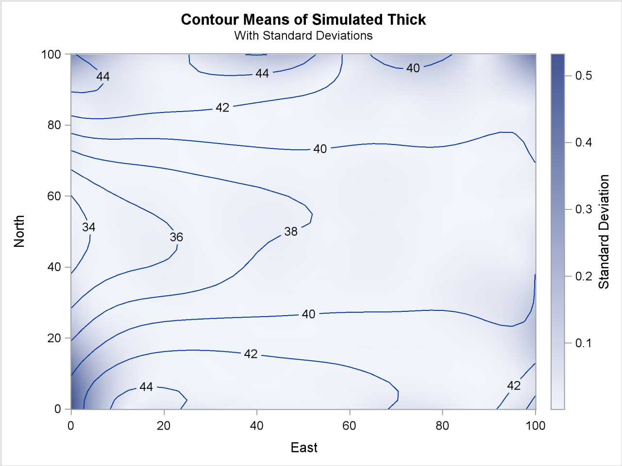
Figure 105.5 Contour Plot of Conditionally Simulated Coal Seam Thickness
