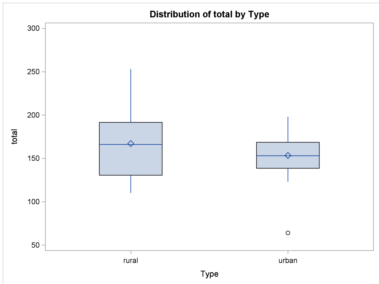
Figure 108.1 Schematic Plots from PROC BOXPLOT
