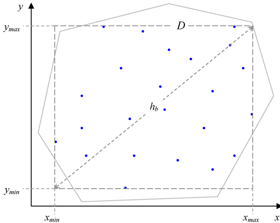
Figure 124.24 Bounding Rectangle to Determine Maximum Pairwise Distance in Domain D
