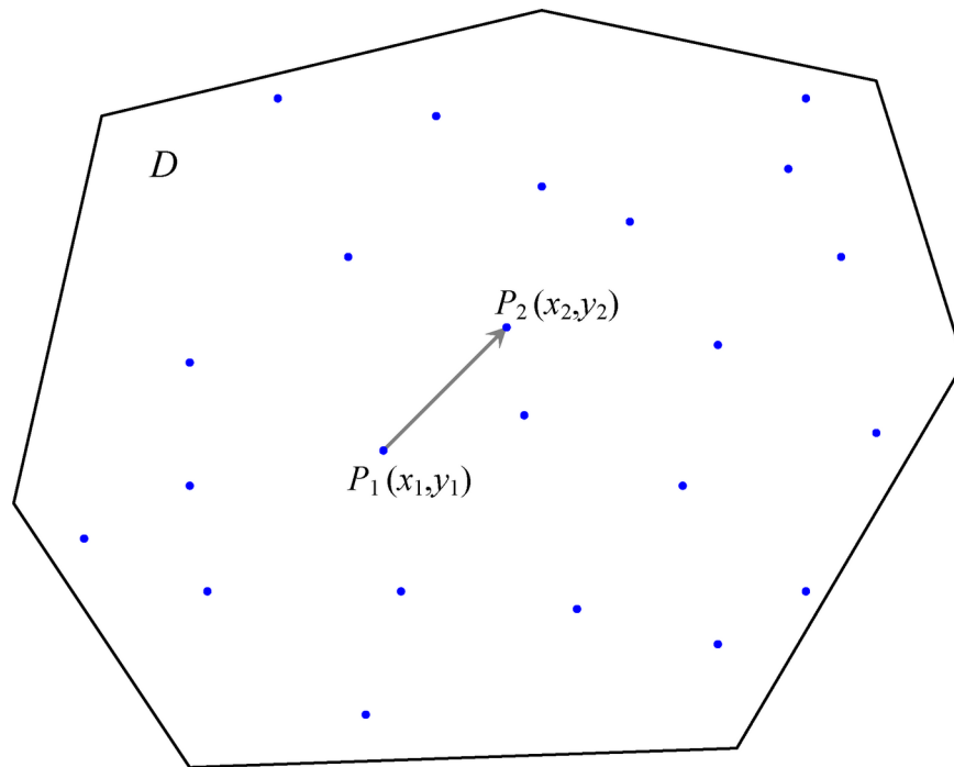
Figure 124.19 Selection of Points P_1 and P_2 in Spatial Domain D
