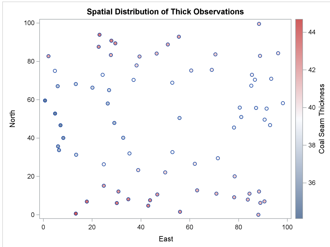
Figure 124.2 Scatter Plot of the Observations Spatial Distribution
