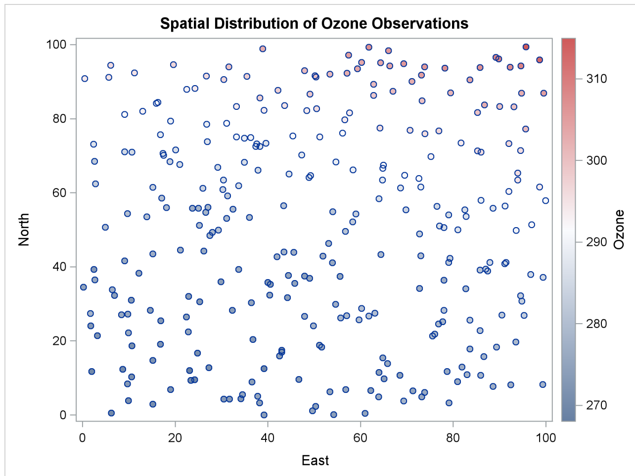
Output 124.2.1 Ozone Observation Data Scatter Plot
