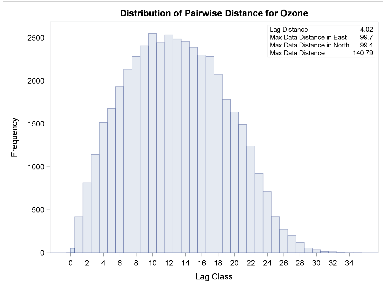
Output 124.2.3 Distribution of Pairwise Distances for Ozone Observation Data
