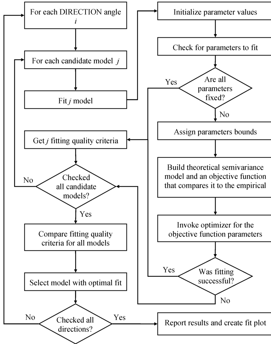
Figure 124.25 Semivariogram Fitting Process Flowchart
