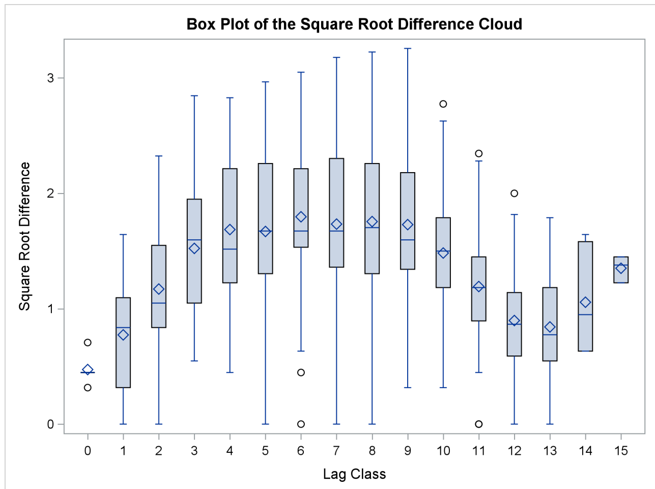
Output 124.5.2 Box Plot of the Square Root Difference Cloud
