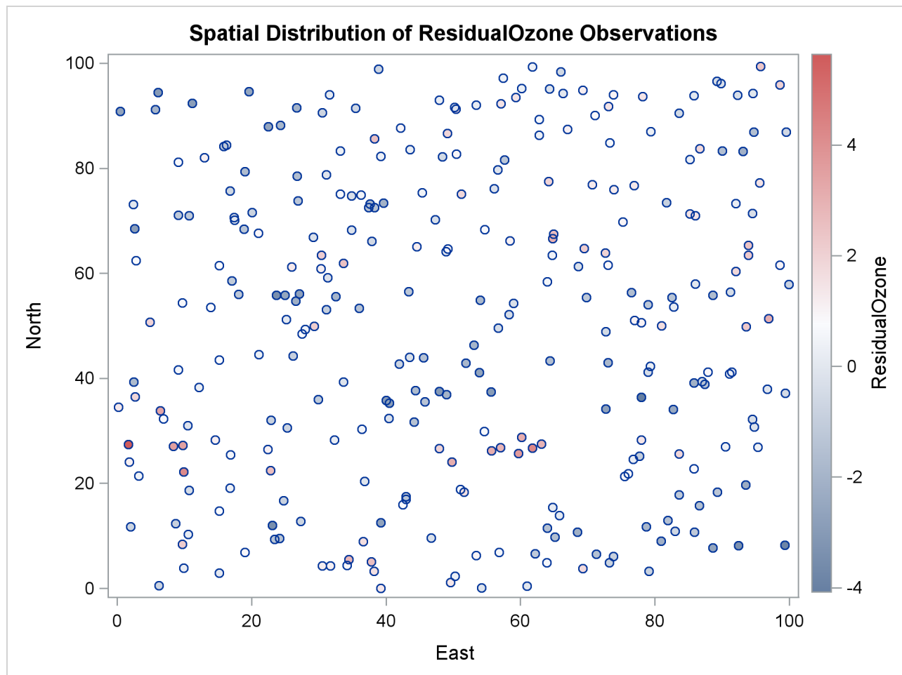
Output 124.2.5 Ozone Residual Observation Data Scatter Plot
