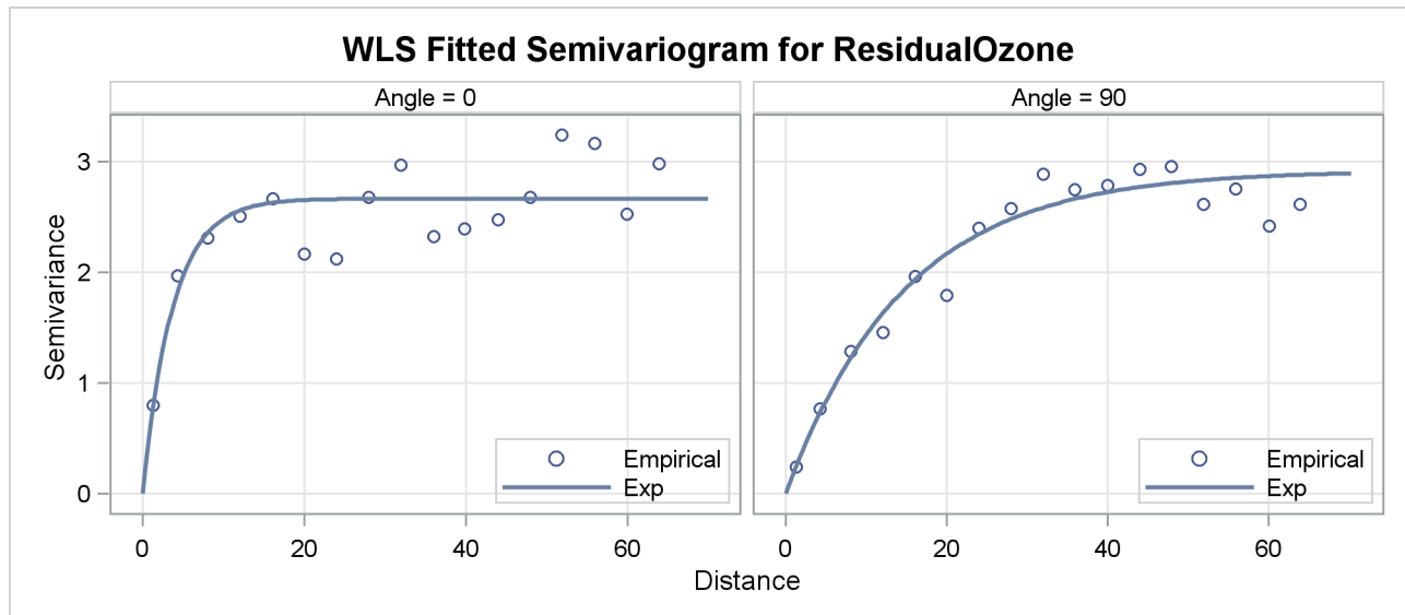
Output 124.2.12 Fitted Theoretical and Empirical Semivariogram for the Ozone Data in the \theta = 0^\circ and \theta = 90^\circ Directions
