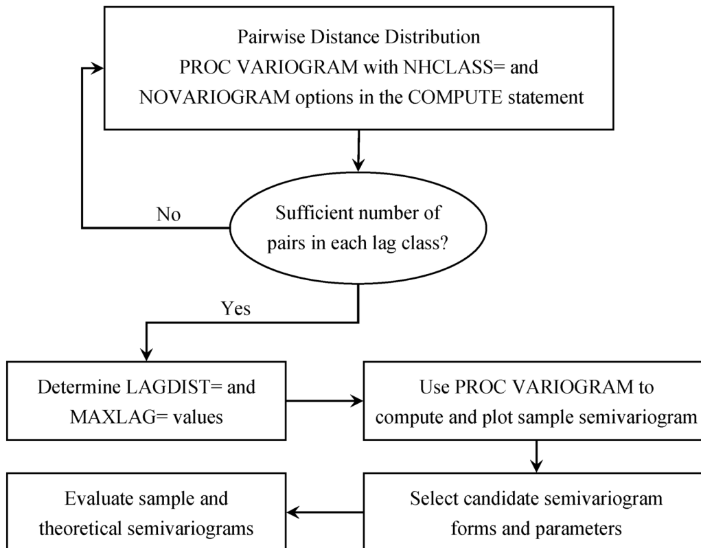
Figure 124.17 Flowchart for Semivariogram Selection
