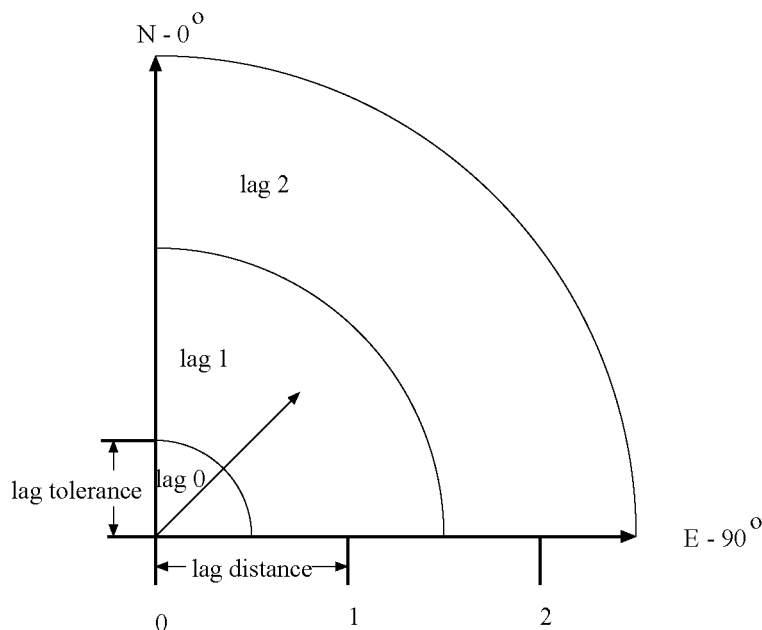
Figure 124.21 Selected Pair P_1 P_2 Falls within the First Lag Class
