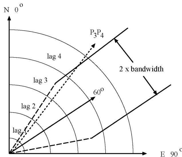
Figure 124.23 Selected Pair P_3 P_4 Falls outside Bandwidth Limit
