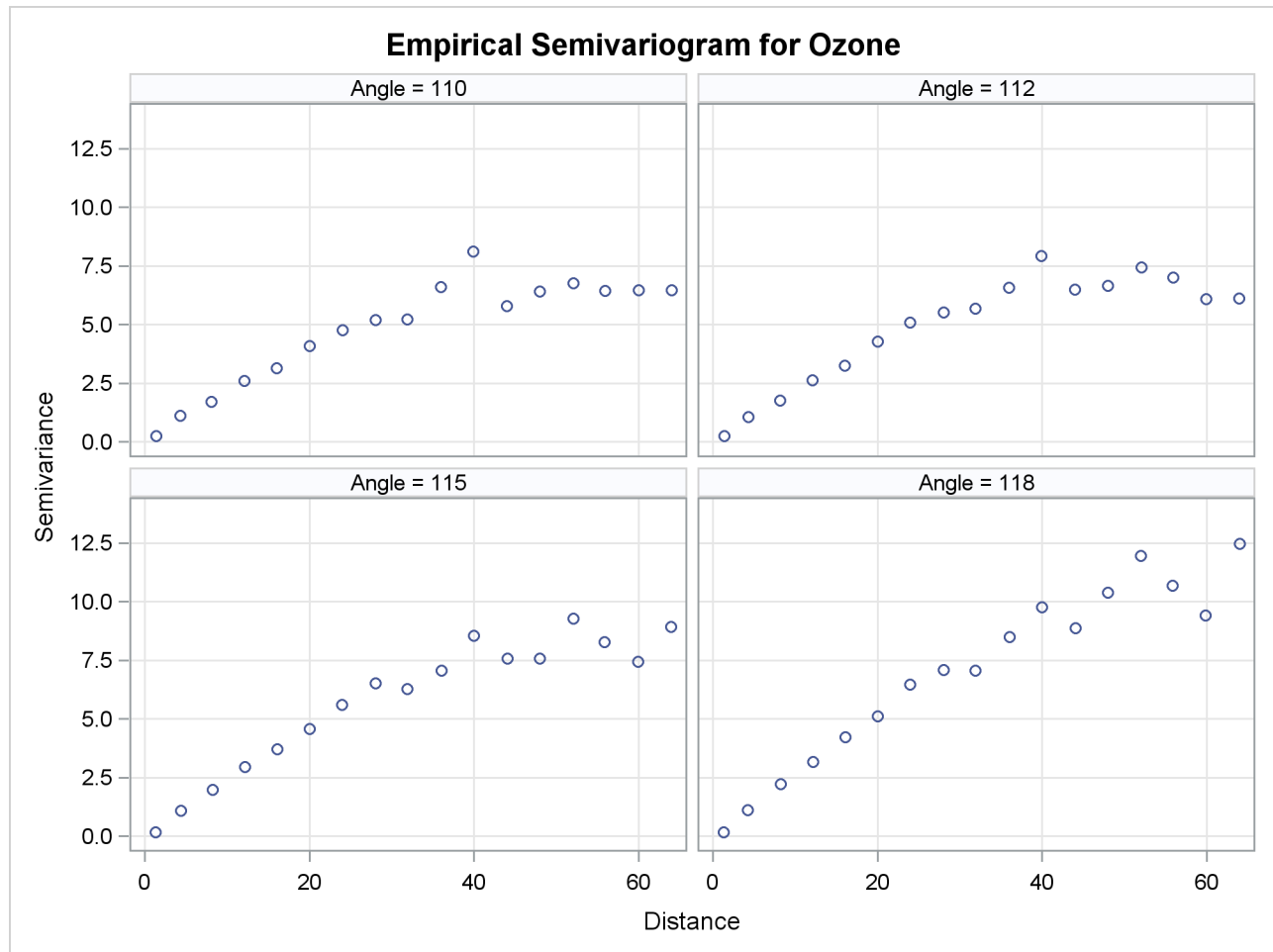
Output 124.3.3 Ozone Empirical Semivariograms in 110°, 112°, 115°, and 118°
