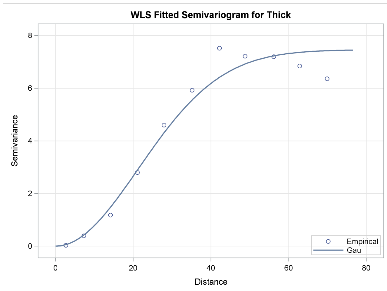
Figure 124.16 Fitted Theoretical and Empirical Semivariogram for Coal Seam Thickness
