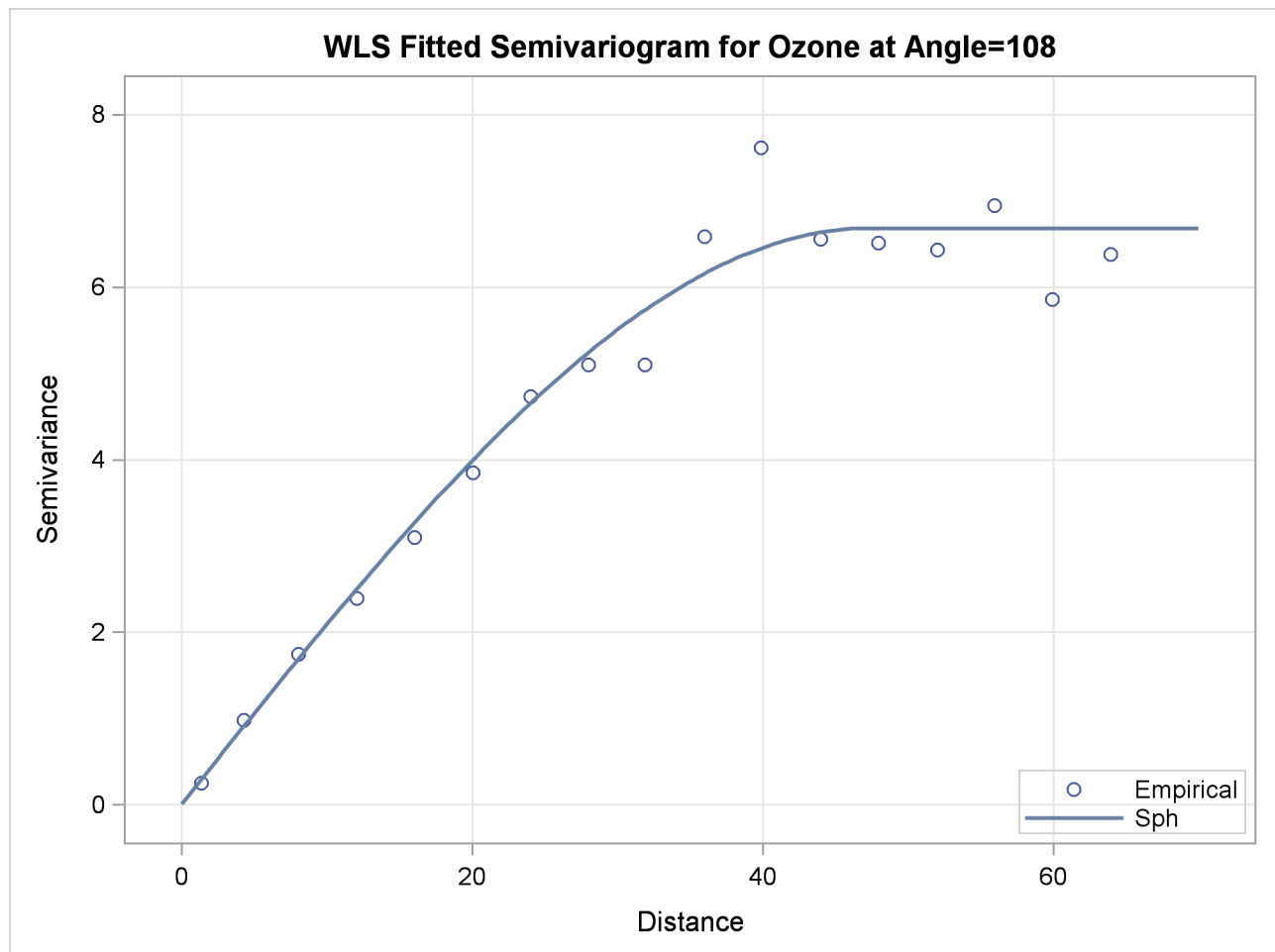
Output 124.3.6 Fitted Theoretical and Empirical Semivariogram for the Ozone Data in \theta = 108^\circ
