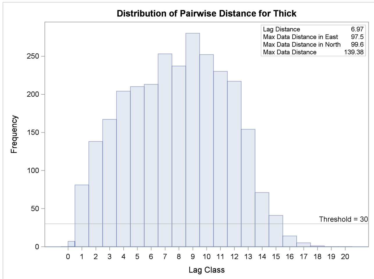
Figure 124.4 Distribution of Pairwise Distances
