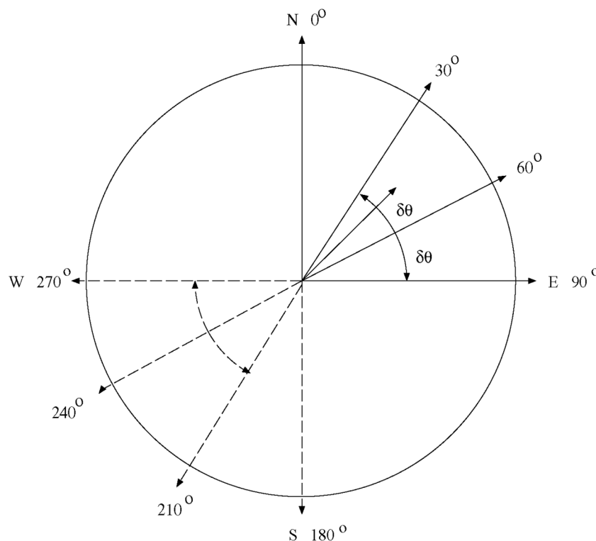
Figure 124.20 Selected Pair P_1P_2 Falls within the Second Angle Class
