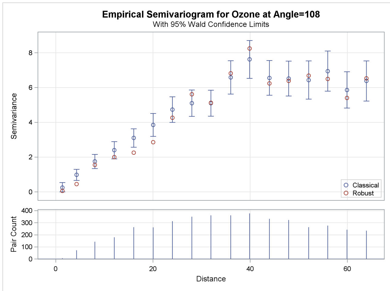
Output 124.3.4 Ozone Classical and Robust Empirical Semivariograms in \theta = 108^\circ
