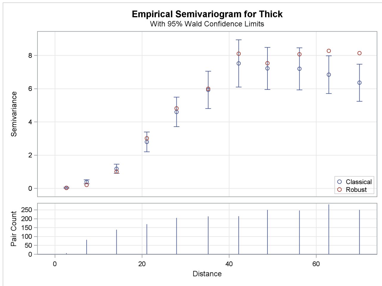
Figure 124.7 Classical and Robust Empirical Semivariograms for Coal Seam Thickness Data
