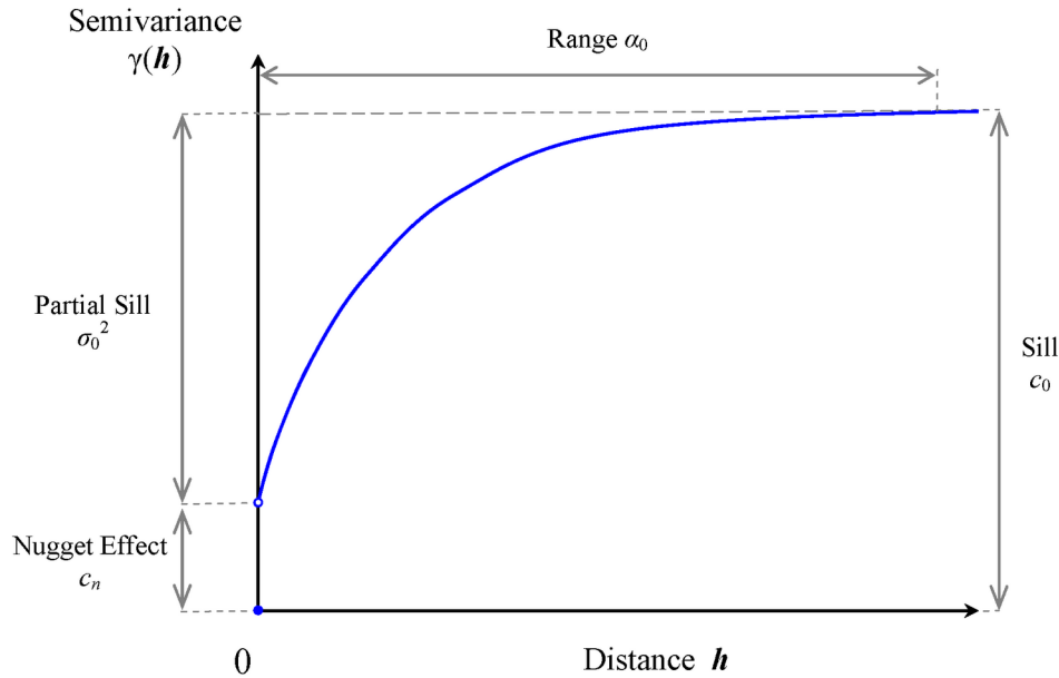
Figure 124.18 A Theoretical Semivariogram of Spherical Type and Its Characteristics
