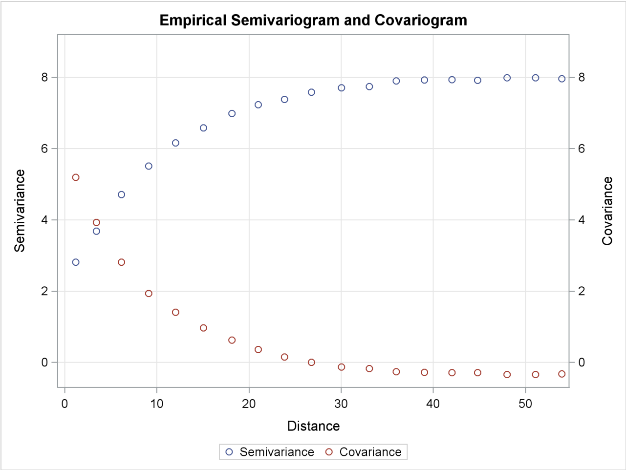
Output 124.4.1 Average Empirical Semivariogram and Covariogram from 500 Simulations
