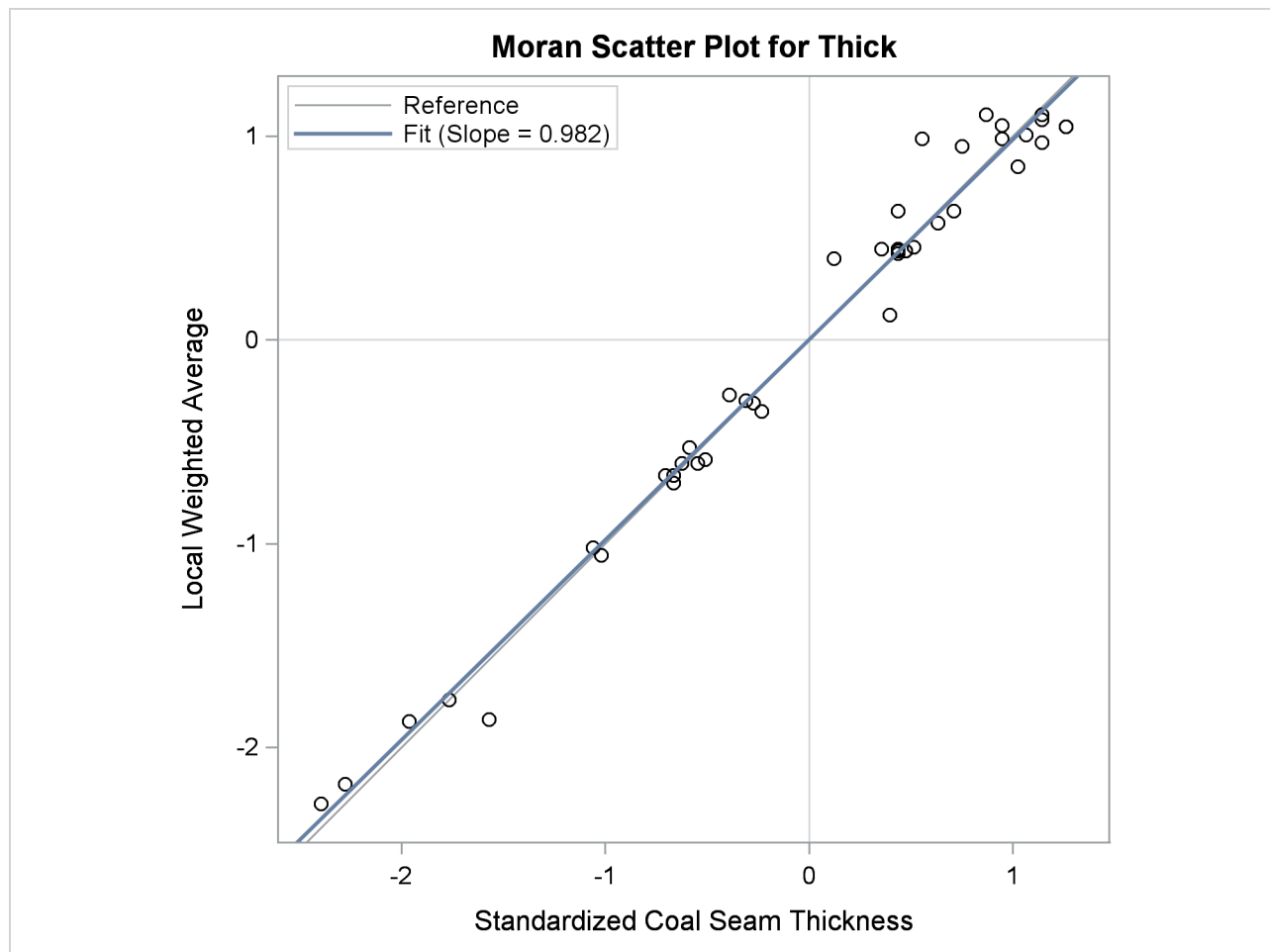
Figure 124.9 Moran Scatter Plot for Coal Seam Thickness Data
