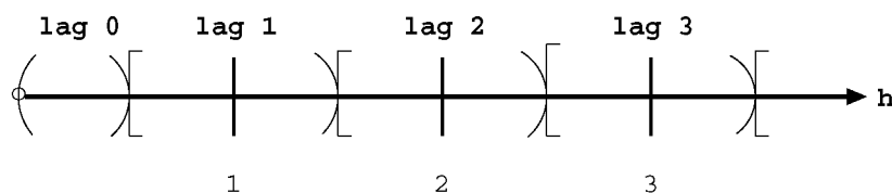
Figure 124.22 Lag Distance Axis Showing Lag Classes
