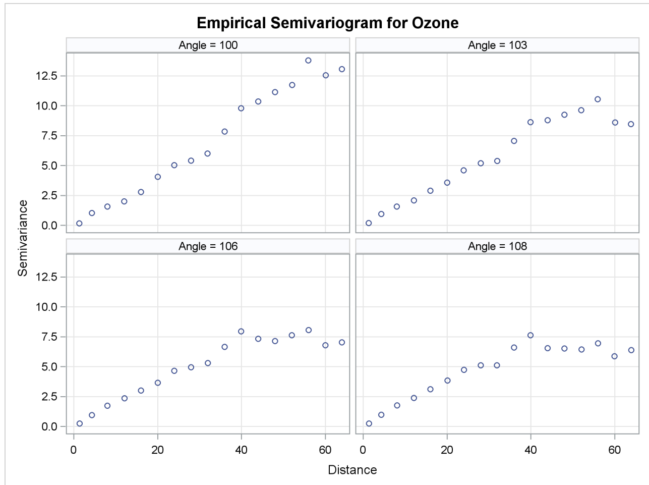
Output 124.3.2 Ozone Empirical Semivariograms in 100^\circ , 103^\circ , 106^\circ , and 108^\circ
