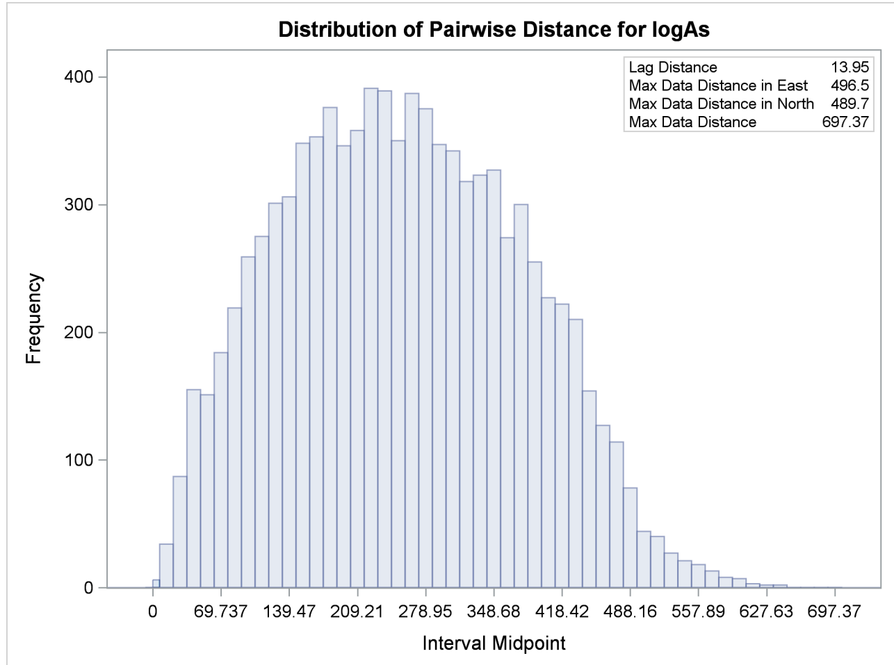
Output 124.1.2 Distribution of Pairwise Distances for logAs Data
