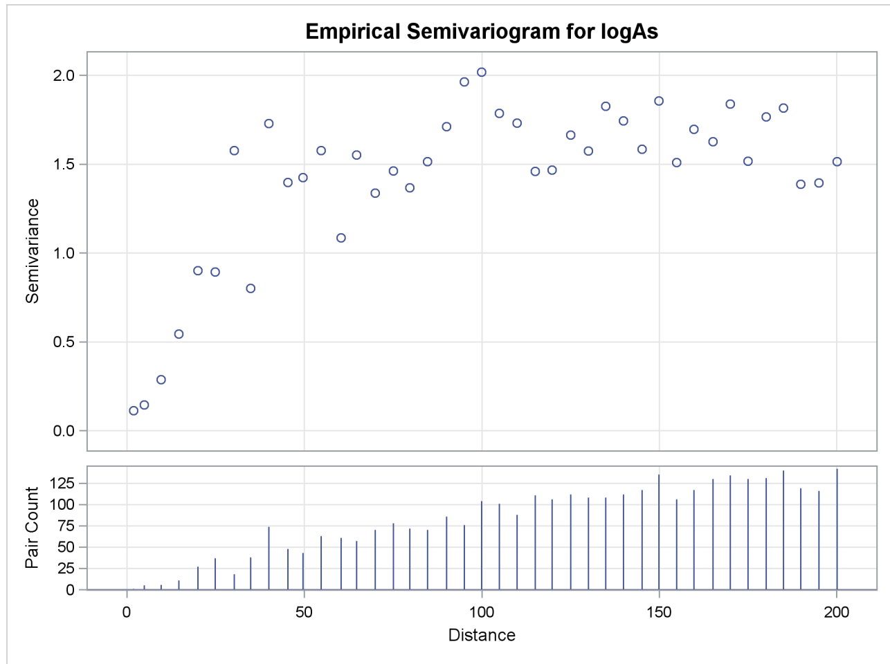
Output 124.1.4 Empirical Semivariogram for logAs Data
