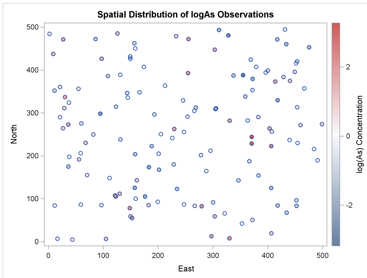
Output 124.1.1 logAs Observation Data Scatter Plot
