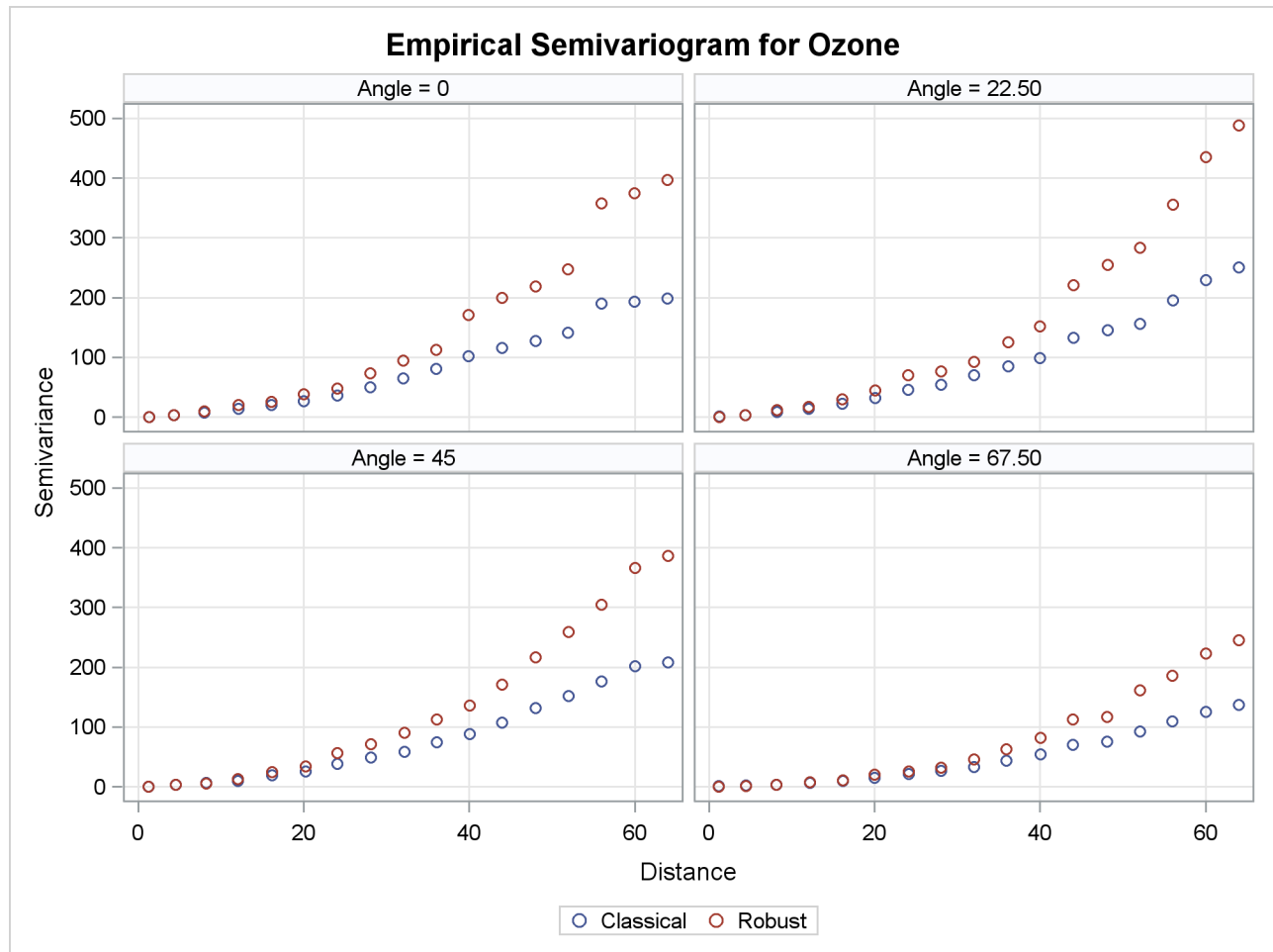
Output 124.3.1 Ozone Empirical Semivariograms with 0^\circ \leq \theta < 180^\circ and \delta\theta = 22.5^\circ
