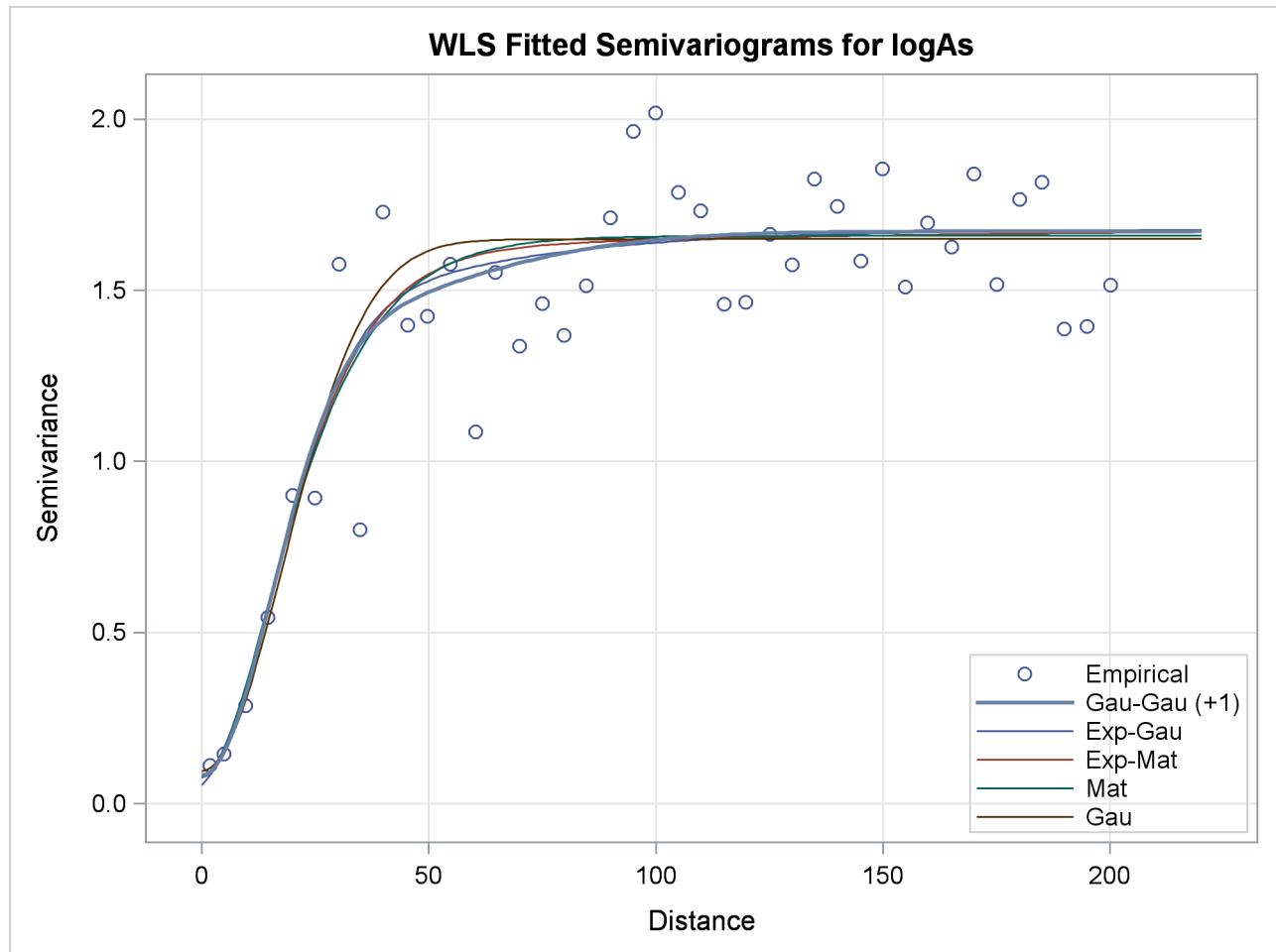
Output 124.1.9 Fitted Theoretical and Empirical logAs Concentration Semivariograms for the Specified Models
