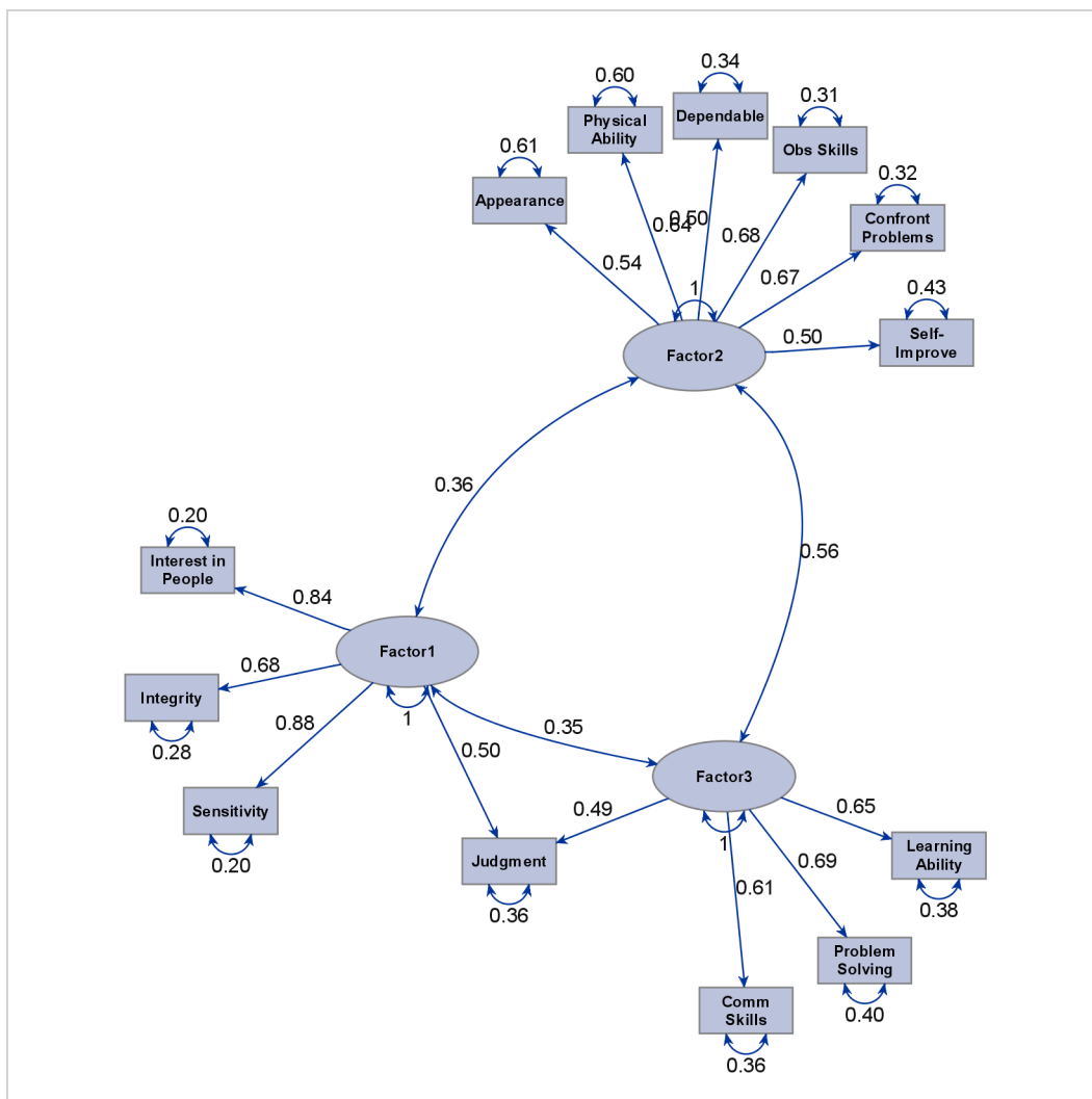
Output 39.6.5 Path Diagram Showing Strong Links by Using the ARRANGE=GRIP Algorithm
