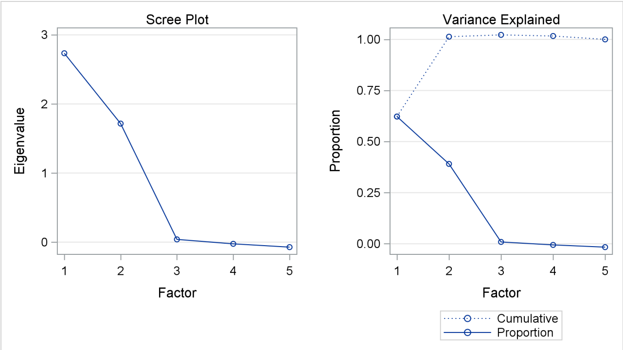
Output 39.2.3 Scree and Variance Explained Plots
