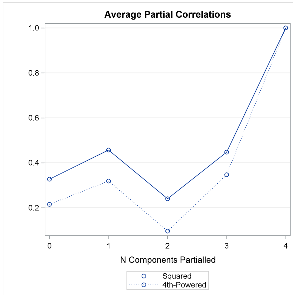
Output 39.3.4 Graphical Summary of the MAP
