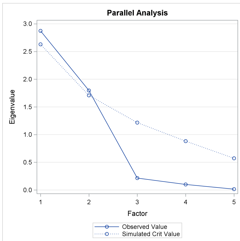
Output 39.3.2 Graphical Summary of the Parallel Analysis
