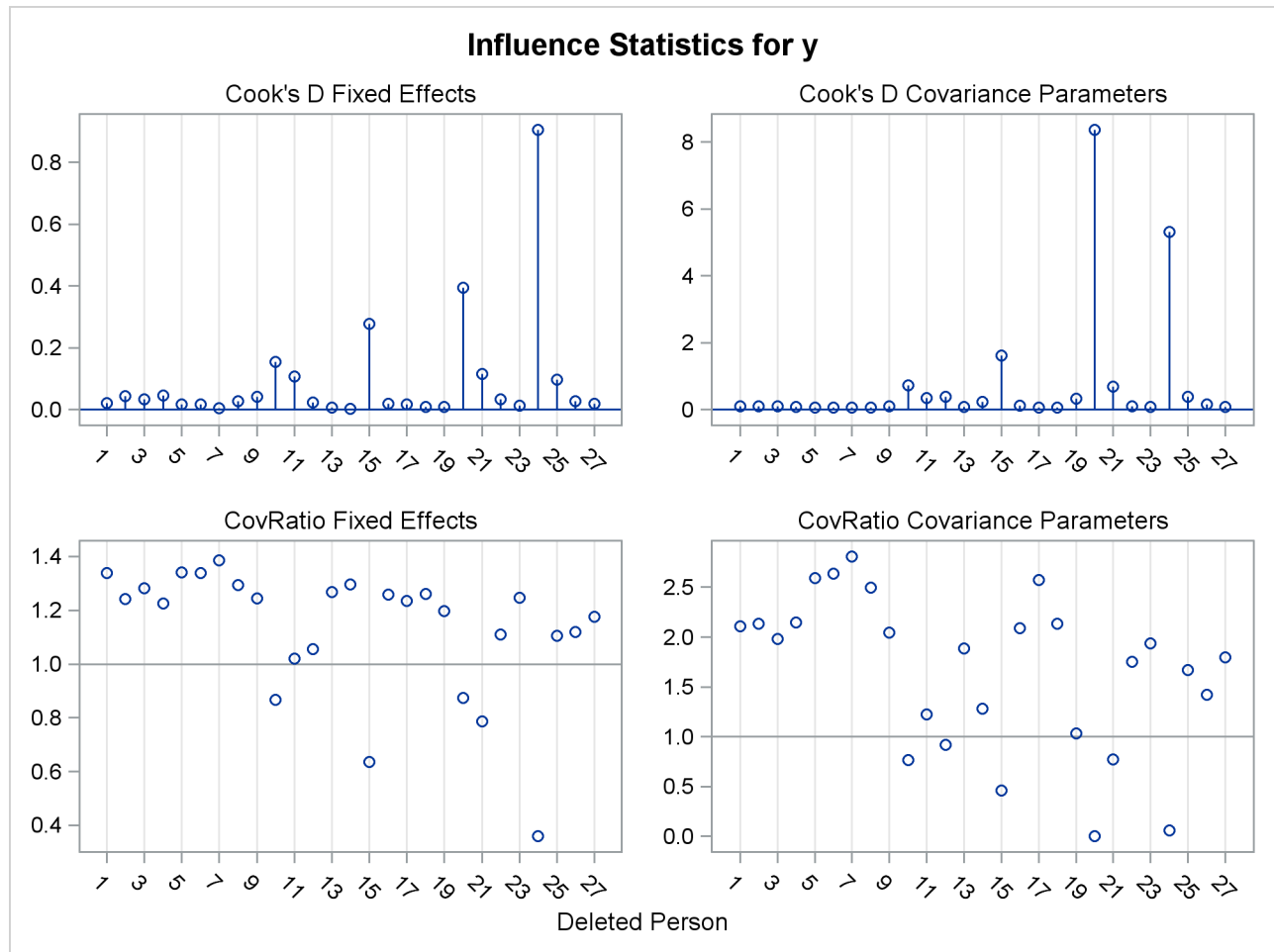
Output 79.8.3 Influence Diagnostics Panel
