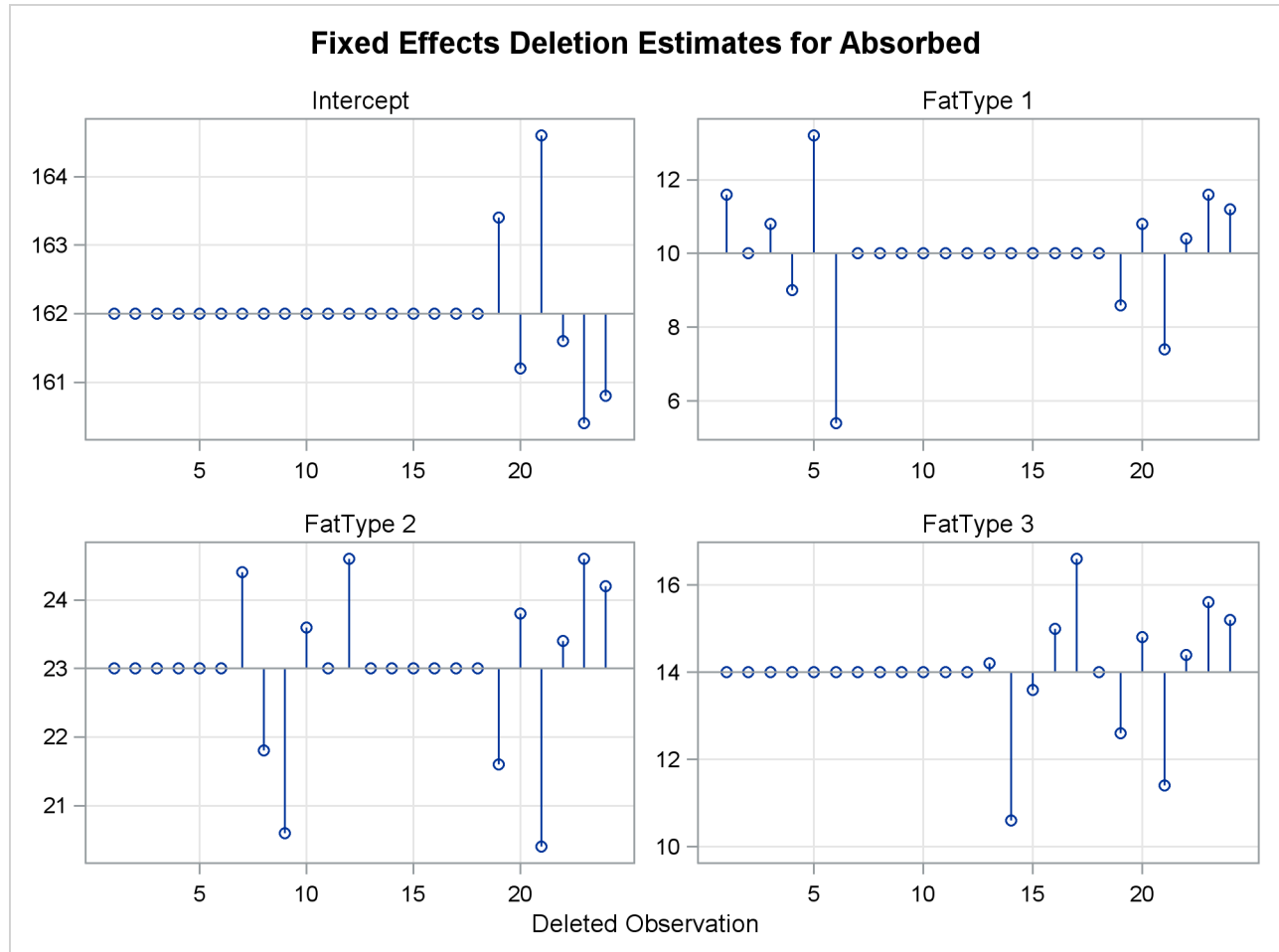
Output 79.7.4 Fixed-Effects Deletion Estimates
